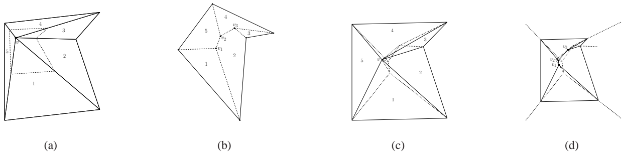
Fig. 6. Changing the initial topology of a vertex of degree greater than 3 (the skeleton is shown in dashed lines). (a) The original polyhedron. Vertex v has degree 5; (b) The cross-section and its weighted straight skeleton. Vertex v becomes three new vertices: v_1 , v_2 , and v_3 ; (c) The straight skeleton of the polyhedron. Vertex v spawned three skeletal edges; (d) The propagated polyhedron. Vertices v_1, v_2, v_3 trace their skeletal edges.
