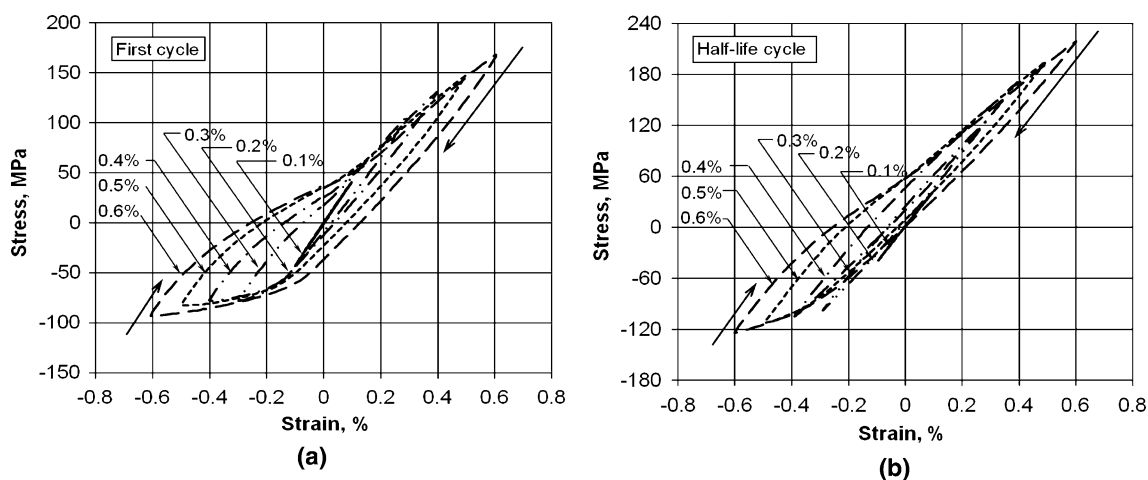
Fig. 8—Hysteresis loops (a) at first cycle and (b) at half-life cycle for different total strain amplitudes.
