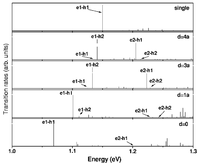
FIG. 10. Electron-hole transition rates for single and several double quantum dots versus separation distance d .
