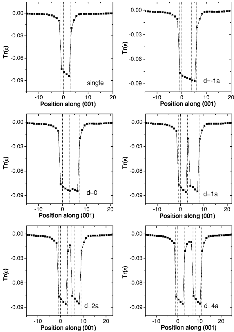
FIG. 1. Trace Tr(\epsilon) of the strain tensor vs cation position (in units of lattice constant) along (001), i.e., along z axis, for a single quantum dot and several double quantum dots. Vertical lines mark WLs and tops of QDs.
