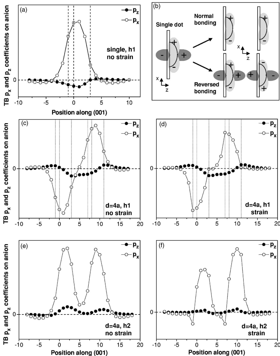
FIG. 8. Spatial envelopes of the p_x and p_z atomic orbital contributions to hole wave functions along (001) at x=0.5a , y=2a : (a) Single QD ground hole state, (c) DQD ( d=4a ) ground hole state h1, no strain effects, (d) DQD ( d=4a ) ground hole state h1 with strain effects, (e) DQD ( d=4a ) first excited hole state h2, no strain effects, (f) DQD ( d=4a ) first excited hole state h2 with strain effects. Full circles indicate p_z contribution, open circles, p_x contributions, respectively. Vertical lines in (a) indicate the wetting layer and the top of the quantum dot. Vertical lines in (c) and (d) indicate the wetting layers and the top of the dots in the DQD. Similar lines should apply for (e) and (f). (b) A scheme showing normal and reverse bonding of the QDs ground hole states.
