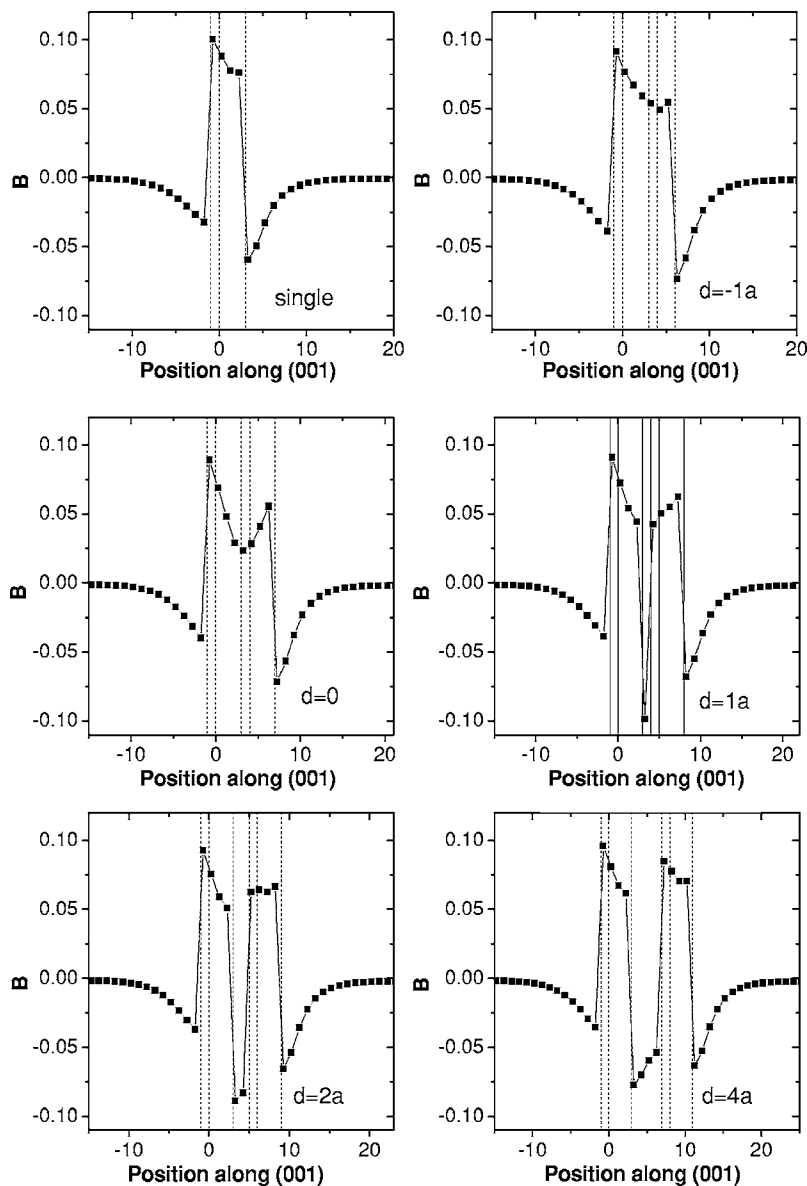
FIG. 2. Biaxial component B of the strain tensor vs cation position (in units of lattice constant) along (001) for a single quantum dot and several double quantum dots. Vertical lines mark WLs and tops of QDs.
