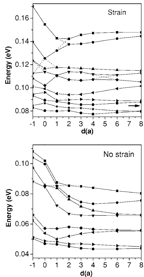
FIG. 5. Dependence of the lowest hole energy levels of a DQD on separation distance d in units of lattice constant. Top—strain effects included, bottom—without strain effects. The arrows mark the WL quasicontinuum of a single QD. Energies are referred to the bulk GaAs valence band edge. Lines connect and order states energetically. Dotted lines show how some states would evolve vs d in the absence of mixing.
