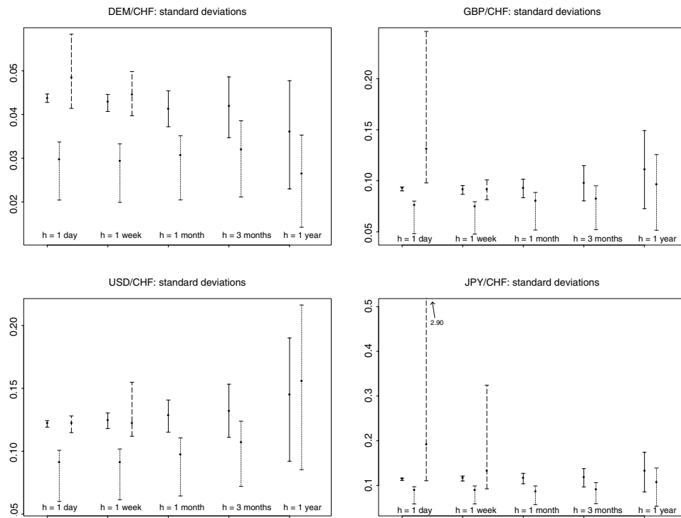
Figure 1. Foreign exchange rates: estimates for standard deviations (including confidence intervals constructed via simulation), using random walk models (full lines), AR(p) models (dotted lines) and GARCH(1,1) models (dashed lines).
