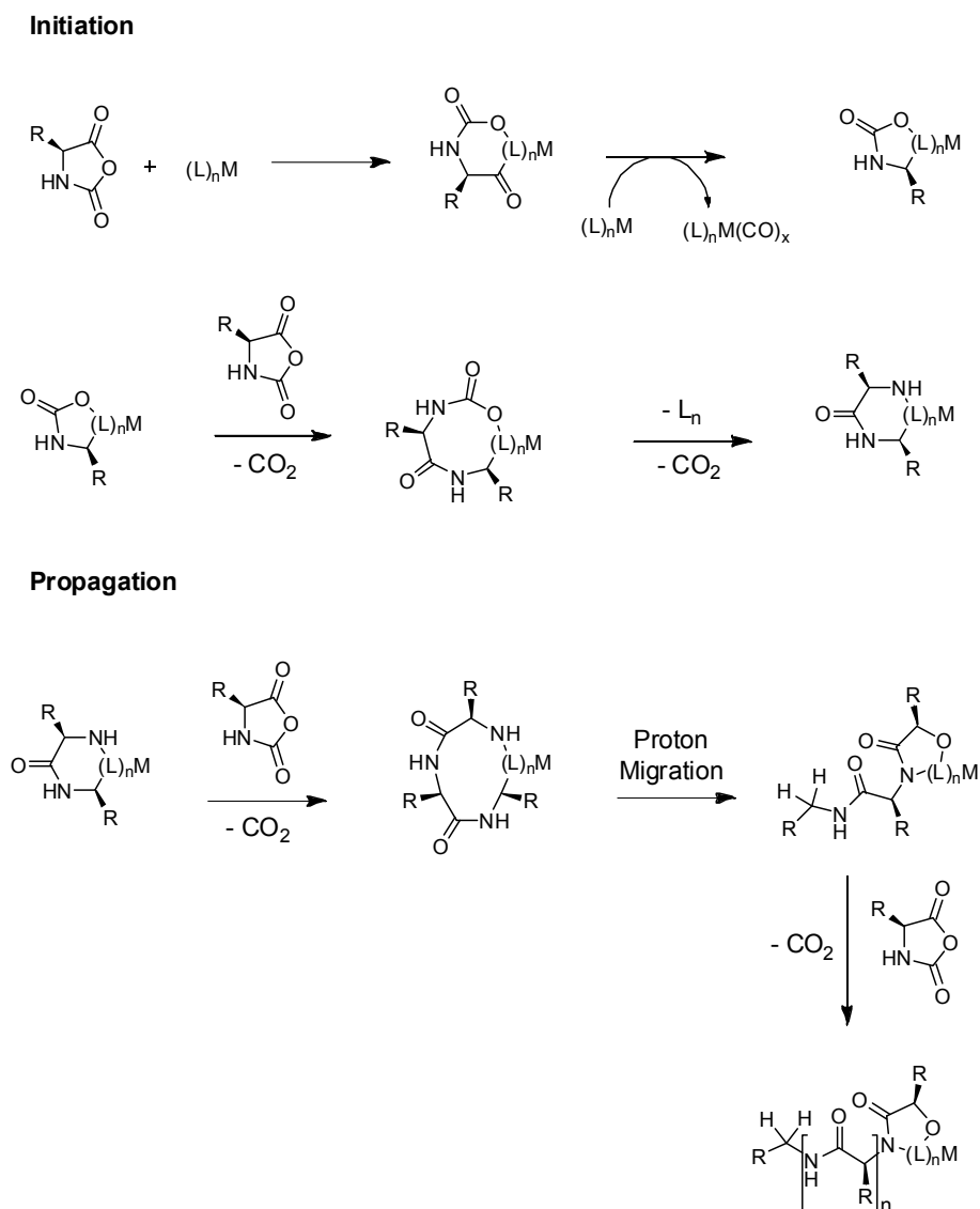
Figure 12. Propagation Reactions of the Mechanism for the Polymerization of NCAs with bipyNi (COD) (bipy) 2,2-bipyridyl, (COD) 1,5-cyclooctadiene) or (\text{PMe}_3)_4\text{Co} complexes proposed by Deming et al. [64–66].
