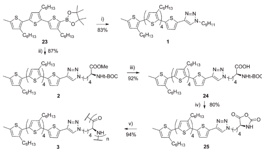
Figure 6. Synthetic route for the preparation of Semiconductor Functionalized Peptide. Reagents and conditions: (i) 12, Pd(PPh 3 ) 4 , K 2 CO 3 , DME, H 2 O, 130 °C, 1 h; (ii) 15, Pd(PPh 3 ) 4 , Cs 2 CO 3 , toluene, reflux, 16 h; (iii) LiOH, THF, H 2 O; (iv) Et 3 N, triphosgene, EtOAc; (v) HMDs, THF, 32 h. Reproduced with permission from reference [53].
