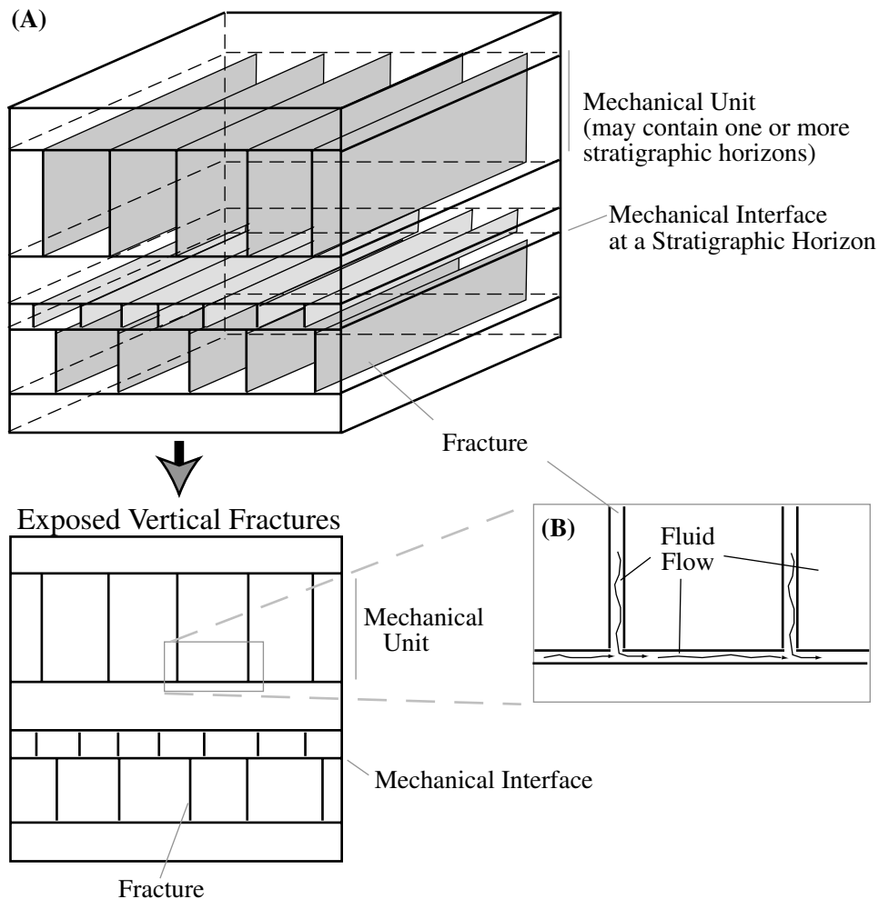
Figure 1. (A) Stratigraphic controls on fracture patterns. Fractures develop within mechanical units and abut mechanical interfaces (modified from Gross et al., 1995). Increased fracture density directly correlates with increased fracture porosity. Both effective porosity and effective permeability are highly dependent on the connectivity of the fracture network; therefore, increased fracture density does not necessarily lead to increased permeability. (B) Termination of vertical fractures can redirect the vertical component of flow to horizontal features, such as dissolutionally enlarged bedding planes. Laterally extensive horizontal high-permeability features are continuous up to 14 km (9 mi) based on hydrogeologic studies of the Silurian dolomite (Muldoon et al., 2001).
