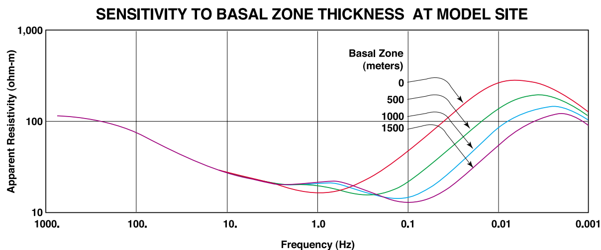
Figure 3: The effect on MT response (apparent resistivity against frequency) of varying the pre-Khuff thickness (fixed at 5 \Omega -m) for the model shown in Figure 2.
