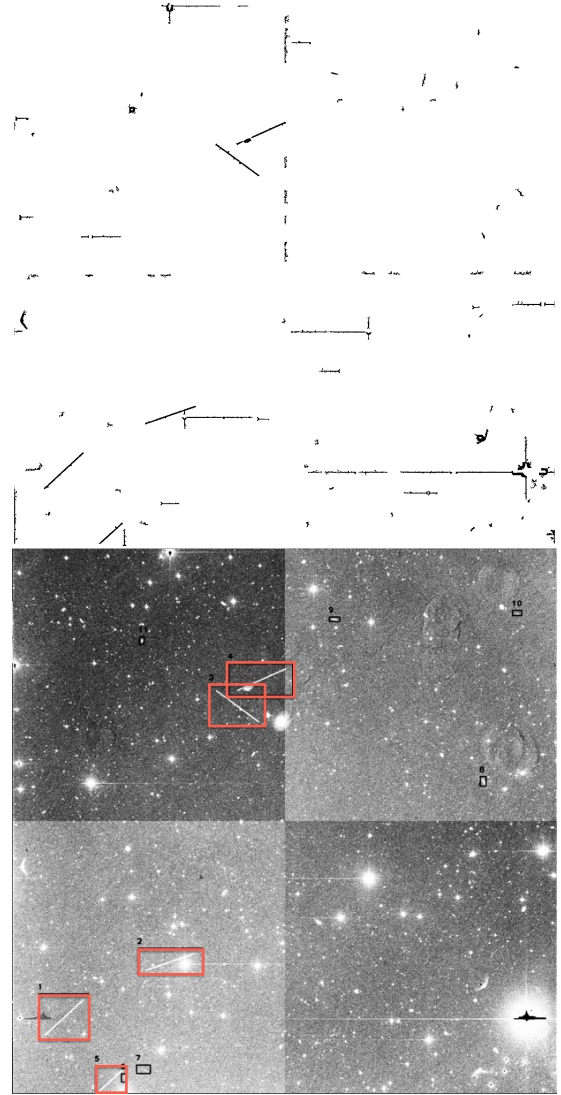
Figure 2. An example for ground-based, sidereal tracking observing scenario: low star density (0.2), long ( L = 200 \text{ px} ) and high ( \text{SNR} \sim 3 ) streaks. Above: segmented image, below: original image with the detected GS streaks (black boxes) and segmented synthetic streaks (red boxes). From Virtanen et al. 2016.
