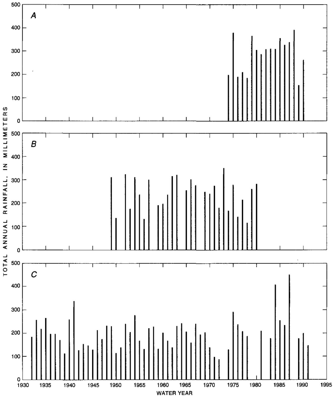
Figure 4. Total annual rainfall for the indicated period for three National Weather Service rainfall-gaging stations, Puerco and Little Colorado River Basins, Arizona and New Mexico. A , Gallup, New Mexico, at Gallup Municipal Airport, water year 1991 incomplete; B , Gallup, water years 1951, 1958, 1964, and 1968 incomplete; C , Holbrook, Arizona, water years 1973, 1979, 1980, 1982, and 1988 incomplete. (Data from the National Oceanic and Atmospheric Administration, National Climatic Data Center.)
