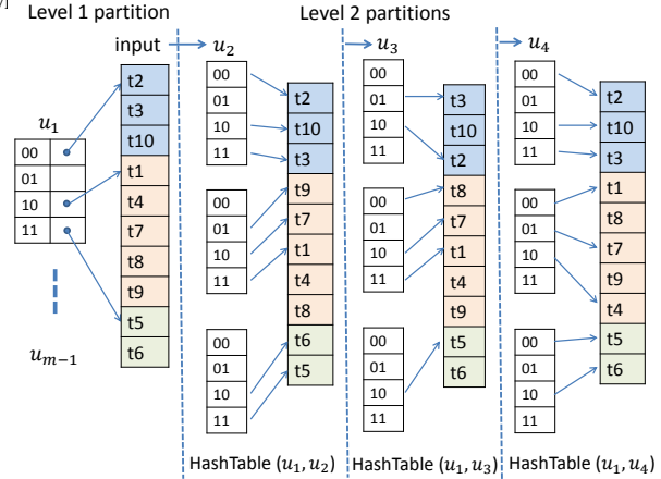
Figure 2: Example with k = 4, m = 4, L = 6 : sharing of the first-level partition among the different hash functions. Hash tables (u_1, u_2) , (u_1, u_3) and (u_1, u_4) are first partitioned according to u_1 . Each partition (shown in different colors) is then partitioned according to hash functions u_2, u_3 and u_4 . The corresponding hash values are shown in Table 1.
