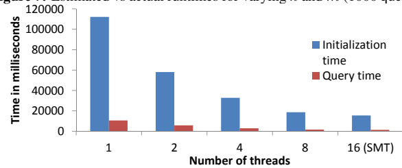
Figure 8: Scaling performance with increasing threads on a single node.
