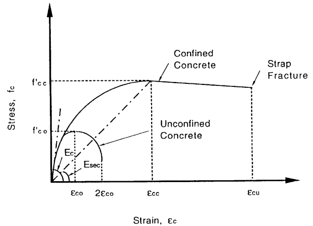
Fig. 3—Stress-strain model proposed for unconfined and confined concrete
