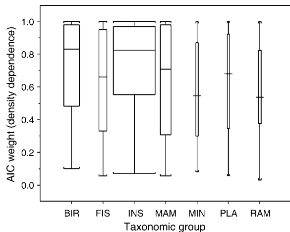
FIG. 1. Distribution of proportional support assigned to density dependence (based on Akaike’s Information Criterion (AIC c ) weights for the three density-dependent models) for birds (BIR), fish (FIS), insects (INS), mammals (MAM), marine invertebrates (MIN), plants (PLA), and reptiles and amphibians (RAM). Bars represent the 50% probability density of the distribution with the width proportional to the number of species in the taxonomic group, black lines indicate the median value, and whiskers show 1.5 times the inter-quartile range.
