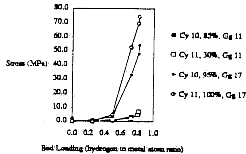
Figure 7. Effect of Unleveling on Wall Stress for Gages 11 and 17 (Level as Indicated). (Bed unleveled before Cycle 11.)
