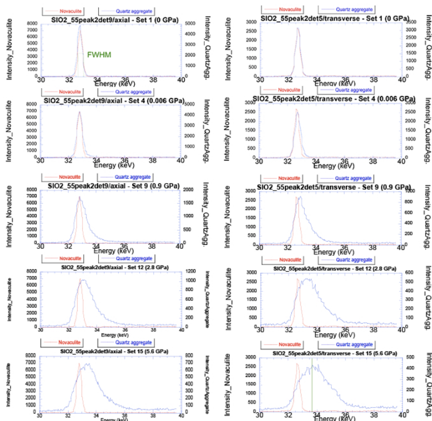
Figure 8: Evolution of the [101] peak for solid grains within quartz aggregate ("quartz agg.") (blue) peaks at selected pressures against the crystallites within the novaculite peak (red) at zero pressure. Both axial (left column) and transverse (right column) directions (experiment SIO2_55) are shown for comparison. This figure has been modified from Cheung et al. 6 Please click here to view a larger version of this figure.
