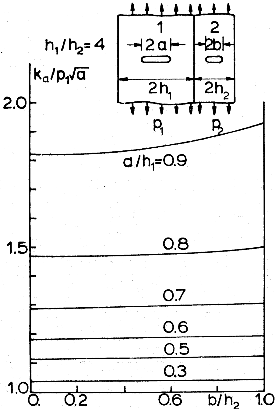
Figure 8. The stress intensity factor k_a for the case in which both strips contain cracks (Combination I).
