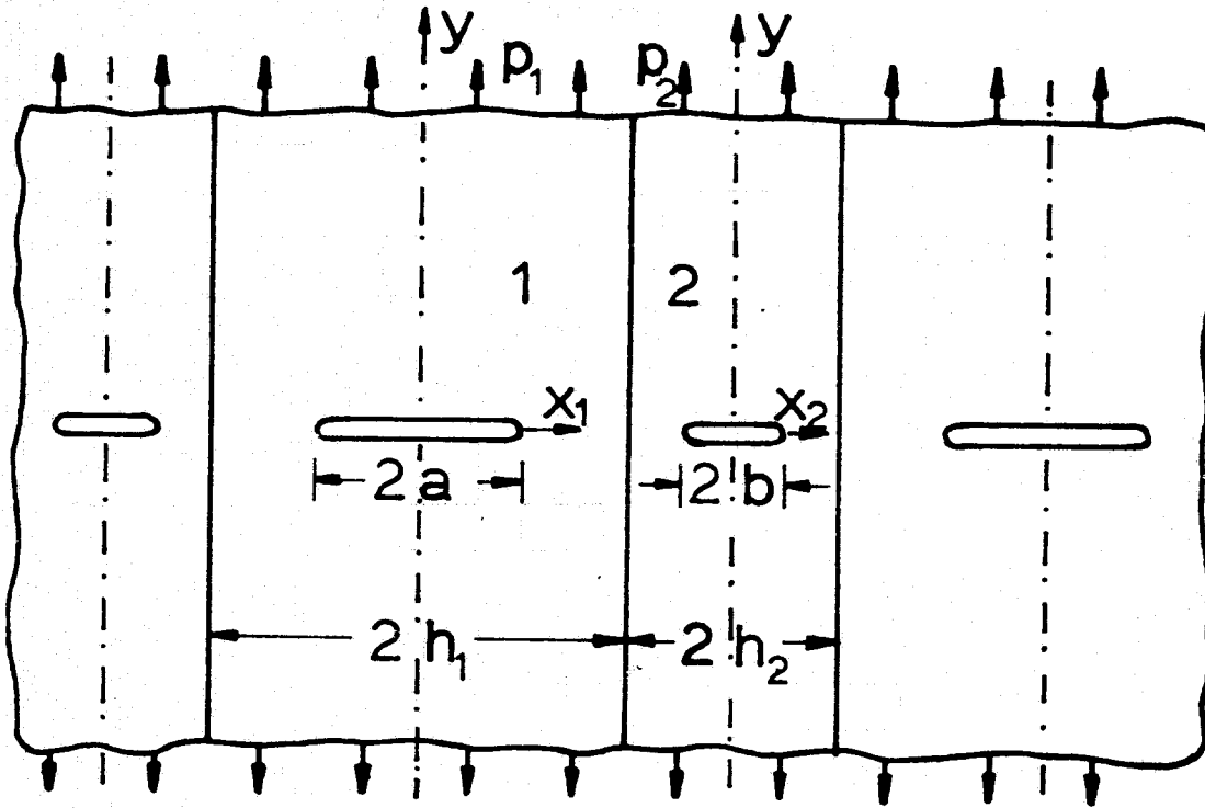
Figure 1. Geometry of the composite plate.
