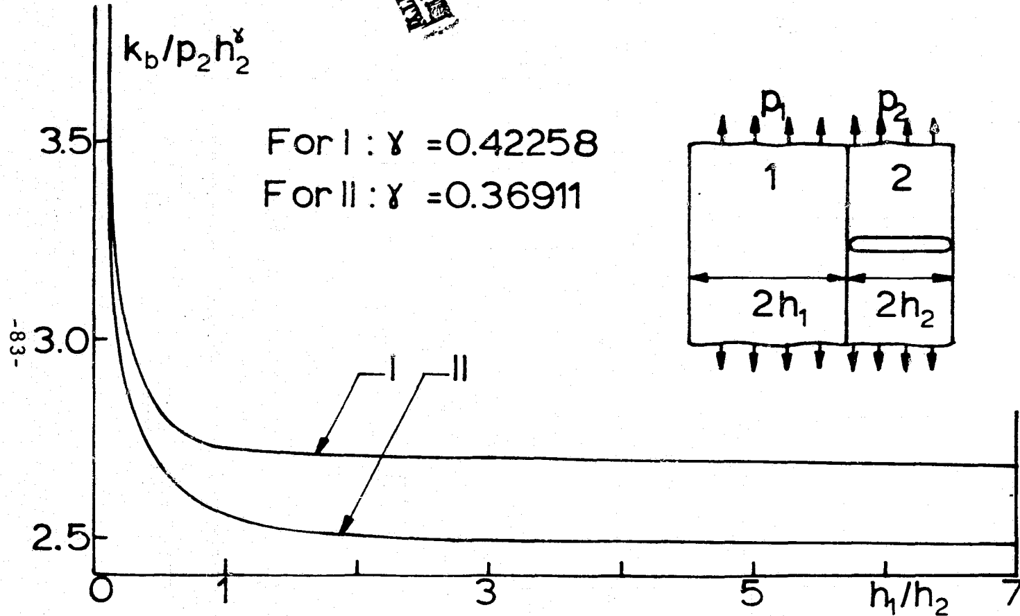
Figure 14. The stress intensity factor k_b when the second laminate is broken (Combination I and II).
