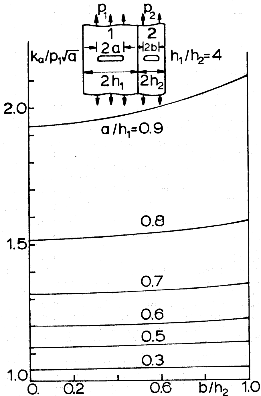
Figure 10. The stress intensity factor k_a for the case in which both strips contain cracks (Combination II).
