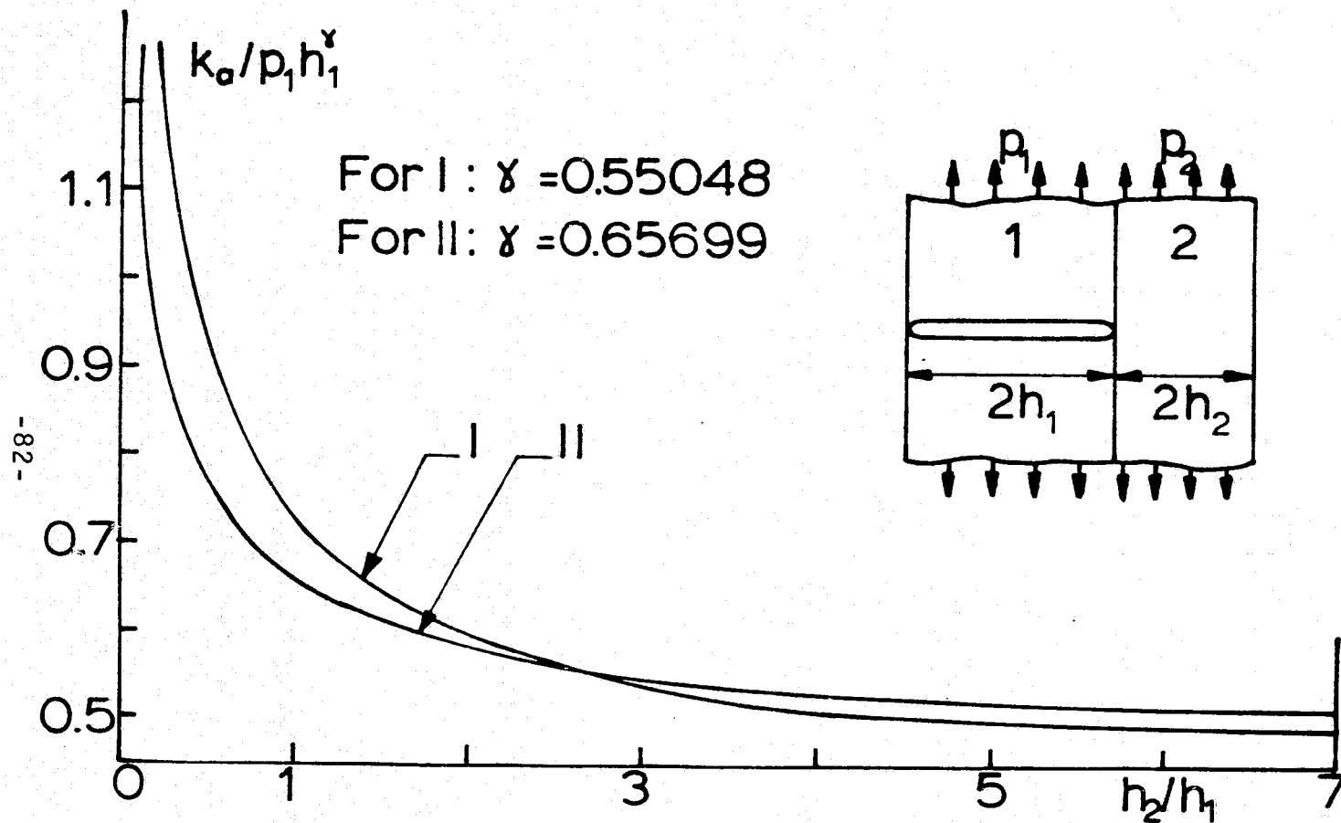
Figure 13. The stress intensity factor k_a when the first laminate is broken (Combination I and II).
