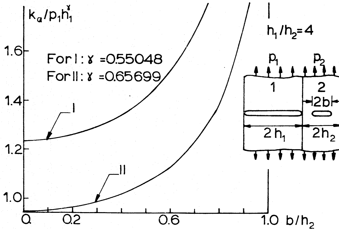
Figure 15. The stress intensity factor k_a when the first laminate is broken and the second contains a crack (Combination I and II).
