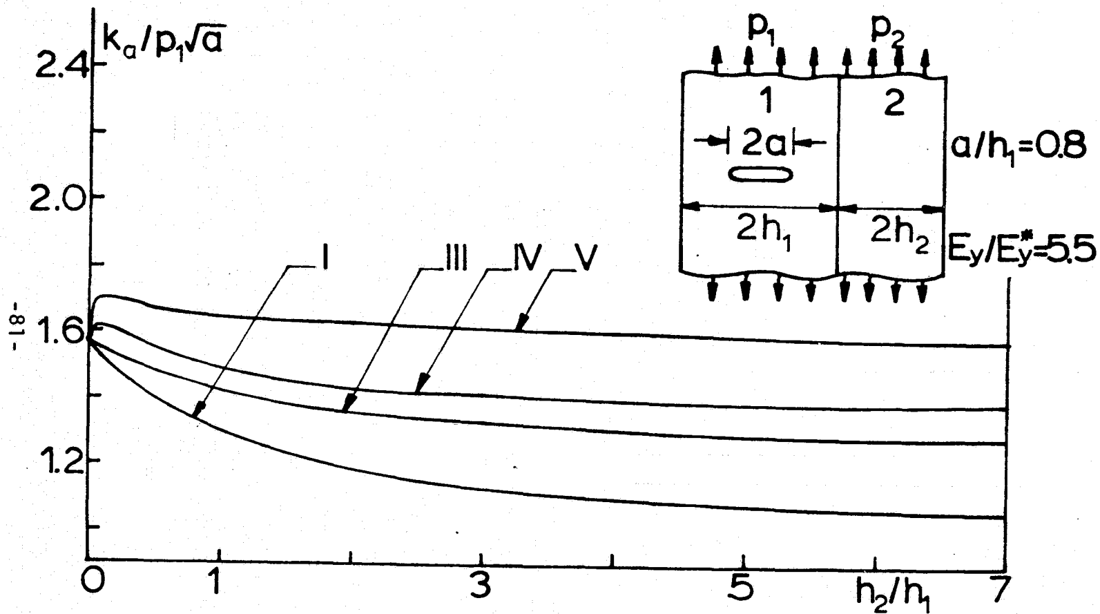
Figure 12. Comparison of the stress intensity factor k_a for isotropic and orthotropic materials.
