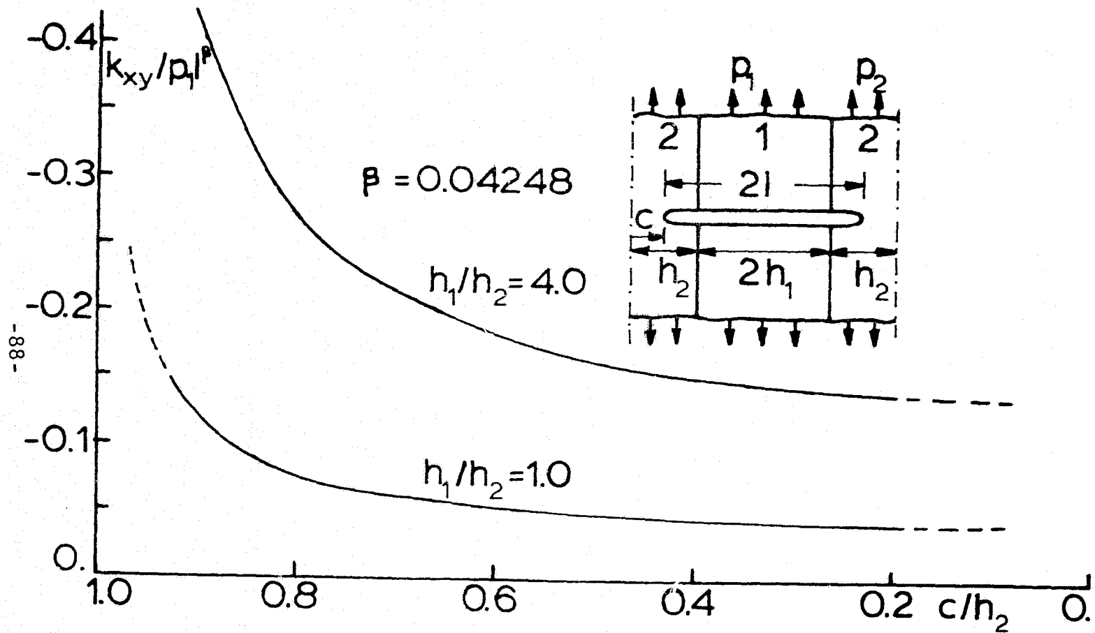
Figure 19. The stress intensity factor k_{xy} for a crack crossing the interface.
