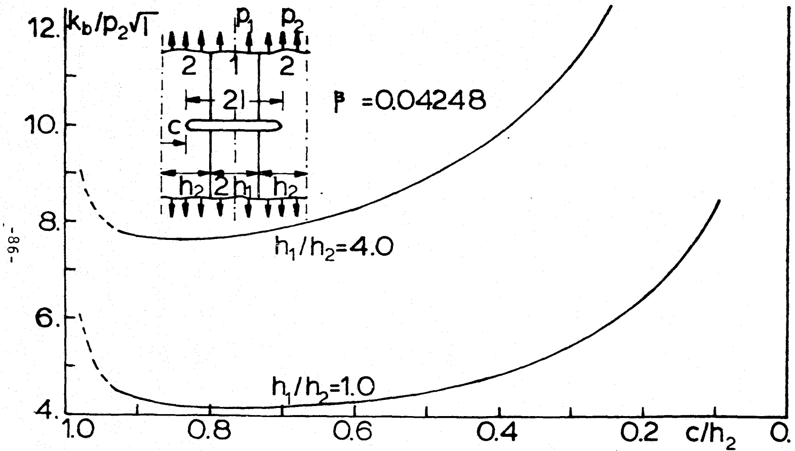
Figure 17. The stress intensity factor k_b for a crack crossing the interface (Singular behavior at the interface).
