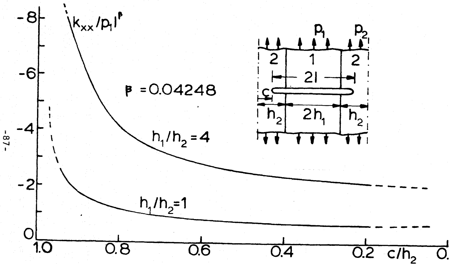
Figure 18. The stress intensity factor k_{xx} for a crack crossing the interface.
