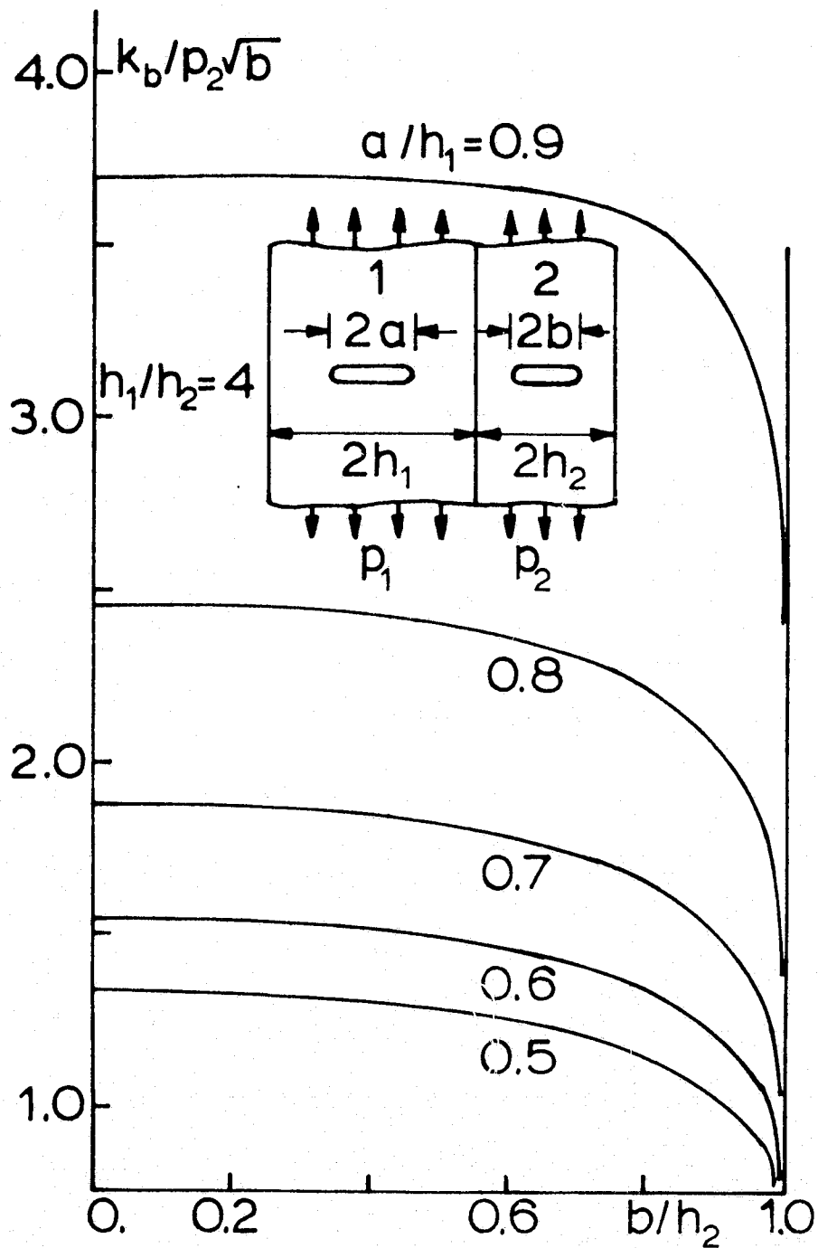
Figure 11. The stress intensity factor k_b for the case in which both strips contain cracks (Combination II).
