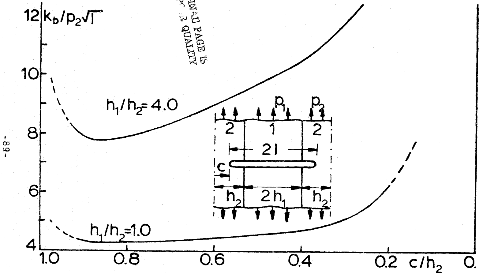
Figure 20. The stress intensity factor k_b for a crack crossing the interface (Non-singular behavior at the interface).
