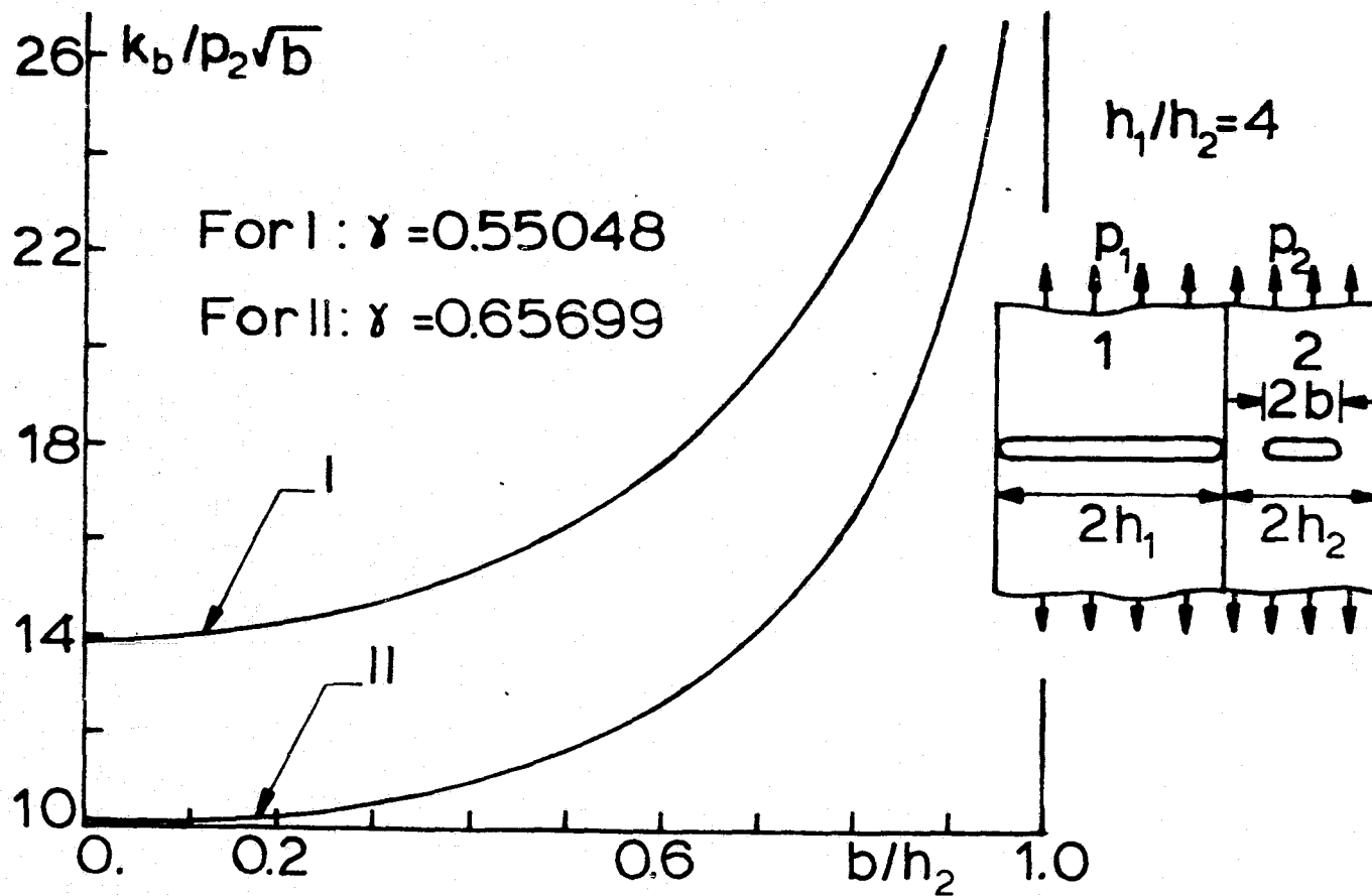
Figure 16. The stress intensity factor k_b when the first laminate is broken and the second contains a crack (Combination I and II).
