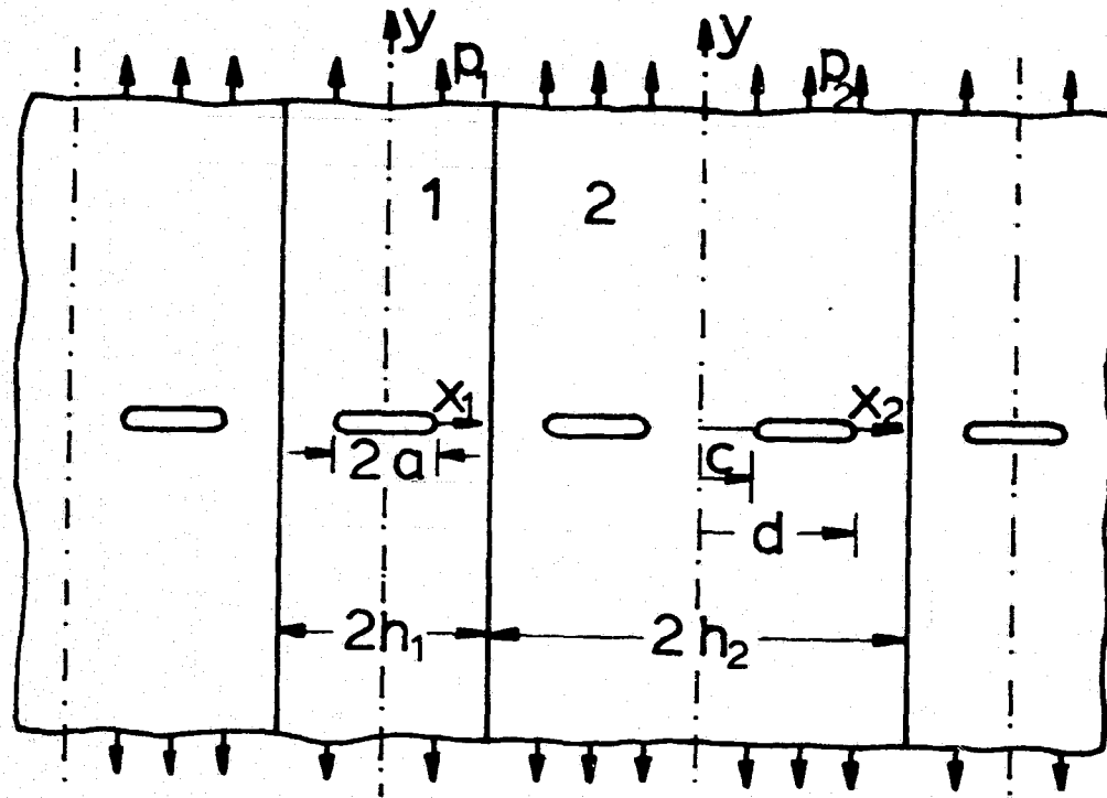
Figure 3. Initial geometry for the case of a crack crossing the interface.
