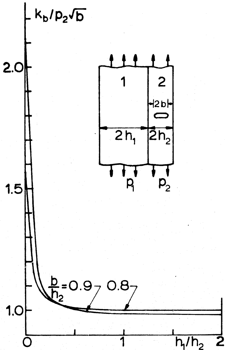
Figure 6. The stress intensity factor k_b for the crack in buffer strip (Combination I).
