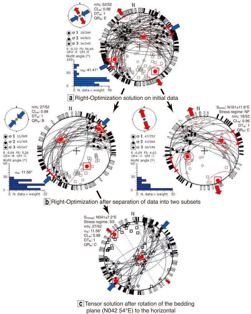
Figure 4. Example of data processing for a measurement site (TO4) in Campanian-Maastrichtian sediments of the Izumi Group (see Figure 1 for site location). (a) Initial data set. (b) Separation of the data into two subsets sorted by mechanical compatibility and field observations. Seven data are rejected in this process. (c) Reduced stress tensor of the first subset after correction of the Izumi Group folding. SS means strike-slip ( \sigma_1, \sigma_3 horizontal), NF normal faulting ( \sigma_2, \sigma_3 horizontal). See text and Table 1 for the definition of other symbols.
