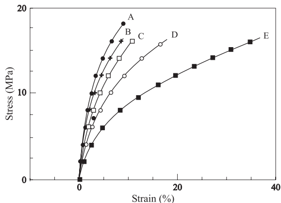
Figure 4. Stress-strain curves of Nafion membranes in different salt forms: (A) (—●—) Nafion-Rb + ; (B) (—+—) Nafion-Cs + ; (C) (—□—) Nafion-K + ; (D) (—○—) Nafion-Na + ; and (E) (—■—) Nafion-Li + .
