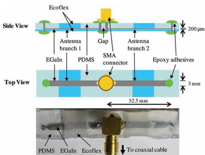
Figure 1. Schematic illustrations and optical micrograph of the stretchable antenna. The half-wave dipole antenna is made of EGaIn embedded in microfluidic channels composed of PDMS and Ecoflex. EGaIn is injected by positive pressure into the inlet, and the EGaIn-filled microfluidic channels are sealed with epoxy resin.
