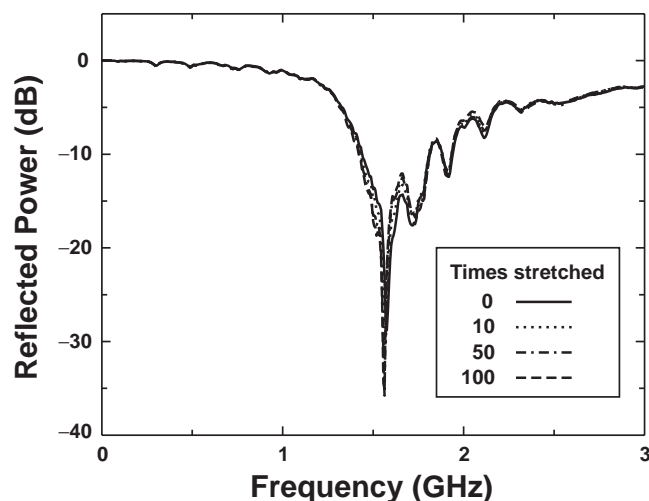
Figure 4. Frequency response of the reflected power from the antenna after repeated stretching up to a strain of 50 %. Plots show the reflected power after the antenna had been stretched 10, 50, and 100 times. The results demonstrated that the resonance frequency and the radiation efficiency of the antenna were almost unchanged (within 1 %) after the antenna had been stretched 100 times.
