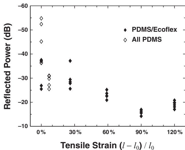
Figure 2. The reflected power (dB) from the antenna as a function of the tensile strain. The filled diamonds show the reflected power of “PDMS/Ecoflex” hybrid structure while the open diamonds show that of “all PDMS” structure at their resonance frequencies. Measurement under each value of strain was repeated five times. The “PDMS/Ecoflex” hybrid structure exhibited good radiation efficiency when stretched up to a strain of 120 %, while the “all PDMS” structure failed at a strain greater than 20 %.
