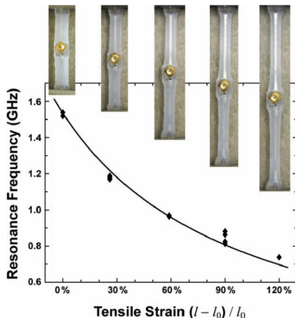
Figure 3. The resonance frequency (GHz) of the antenna as a function of the tensile strain. The resonance frequency of the antenna decreased from 1.53 GHz to 0.738 GHz as the antenna was stretched from l_0 to l = 2.20 l_0 . After releasing the strain, the resonant frequency returned from 0.738 GHz to 1.53 GHz: the tuning is thus reversible. Measurement under each value of strain was repeated five times; and the data points are shown as individual diamonds ( \diamond ) in the plot. The fitted curve was calculated using Equation (1) with \epsilon_{\text{eff}} = 2.1 .
