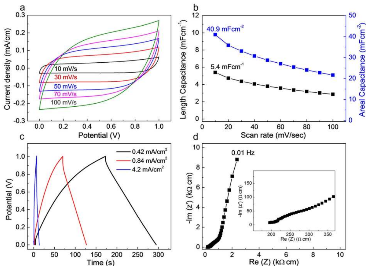
Figure 2 | Electrochemical performance of the solid-state MnO 2 /CNT/nylon fiber supercapacitor. (a), CV curves measured from 10 to 100 mV/s for a solid-state MnO 2 /CNT/nylon fiber supercapacitor. The supercapacitor consists of two symmetrical coiled electrodes coated by PVA-LiCl gel electrolyte. (b), Calculated linear capacitance (normalized by supercapacitor length) and areal specific capacitance (normalized by the surface area of the MnO 2 /CNT/nylon electrode) as a function of voltage scan rate. (c), Galvano-static charge/discharge curves measured for from 0.42 mA/cm 2 to 4.2 mA/cm 2 current densities. (d), Nyquist curve for the frequency range from 0.01 to 1 kHz (the inset shows the high frequency region). The length of the supercapacitor for Fig. 2 measurements was 1 cm.
