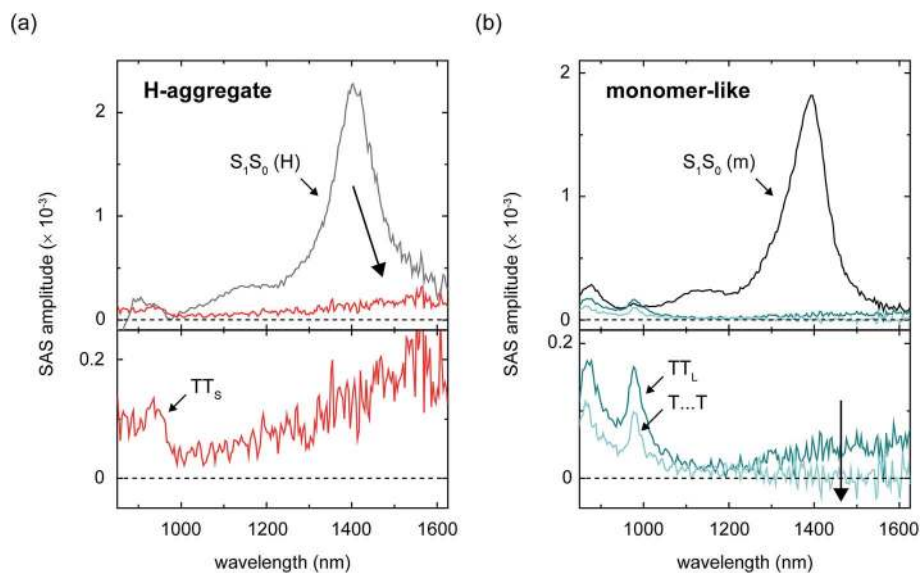
Fig. 7 Near-infrared species-associated spectra derived from a six-component global target analysis of amorphous TIPS-Pn films associated with the set of parent singlet excitons and nascent triplet pairs populated at dimer pair sites comprising chromophores that are (a) H-aggregated and (b) monomer-like. The species-associated spectrum for the short-lived nascent triplet pair preceding intermolecular structural relaxation ( i.e. , SAS-3 or TT*) has been omitted for clarity. The large arrows highlight the signal amplitude in the vicinity of ca. 1600 nm that is apparent in the nascent triplet pair populations, but not in the spatially separated triplet pairs.
