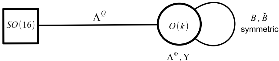
Figure 3: The quiver for \mathcal{O}(-1) \rightarrow \mathbb{P}^1 strings.
