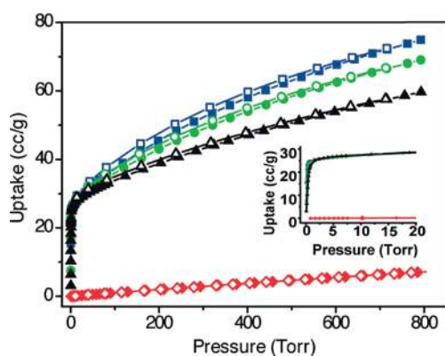
Figure 2. Gas adsorption isotherms for activated CD-MOF-2, illustrating the uptake of \text{CO}_2 measured consecutively at 273 K (blue squares), 283 K (green circles), and 298 K (black triangles) to be contrasted with the uptake of \text{CH}_4 at 298 K (red diamonds). Solid symbols indicate gas sorption and open symbols gas desorption. The initial steep rises observed at very low \text{CO}_2 pressures reach the same value of \sim 23 cc/g regardless of temperature and are believed to be characteristic of a chemisorption process. 11
