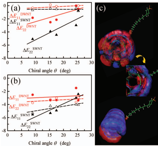
FIG. 2. (Color) (a) The difference of E_{11}^S and E_{22}^S transitions by changing surfactants from (a) SDS to SDBS and (b) SDBS to PVP as a function of chiral angle. (c) The charge density distributions of the (10,2) SWNT and (10,2) at (16,6) DWNT by attaching a SDBS molecule. The inset of (c) is an enlarged image of inner tube of the DWNT near the point to the adjacent SDBS.
