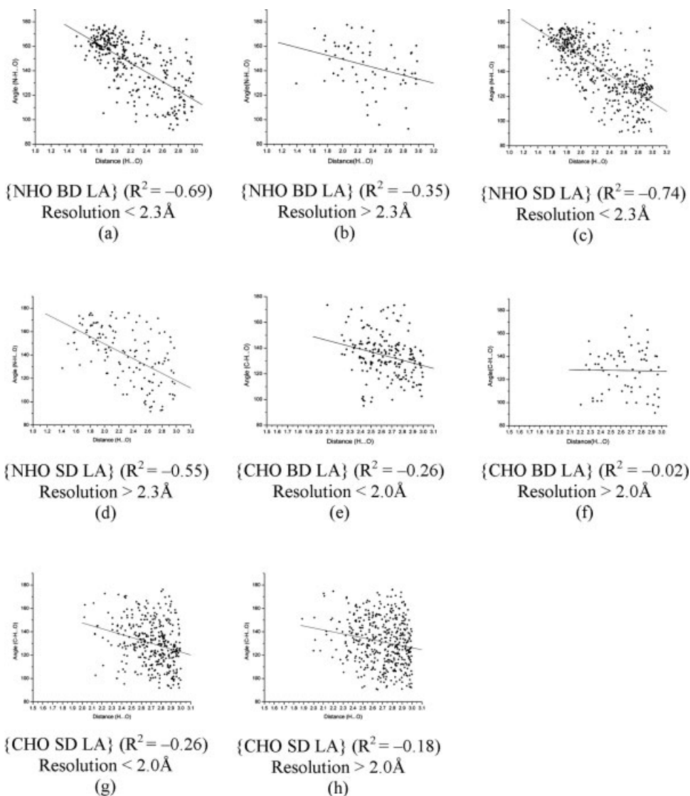
Fig. 6. d=0 Scatterplots for \{NHO\ BD\ LA\} , \{NHO\ SD\ LA\} (a)–(d), and \{CHO\ BD\ LA\} , \{CHO\ SD\ LA\} (e)–(h). Notice the different appearance of these two sets of plots below and above the threshold resolution limits.
