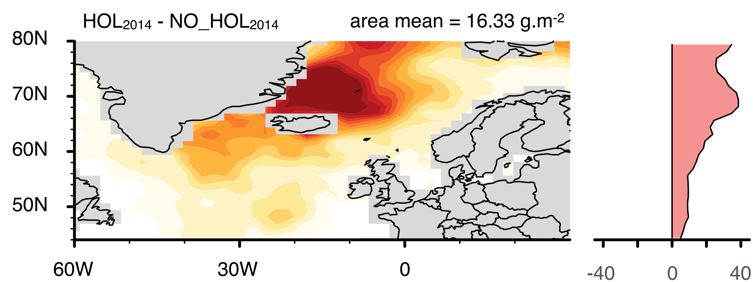
CAM5-Oslo
