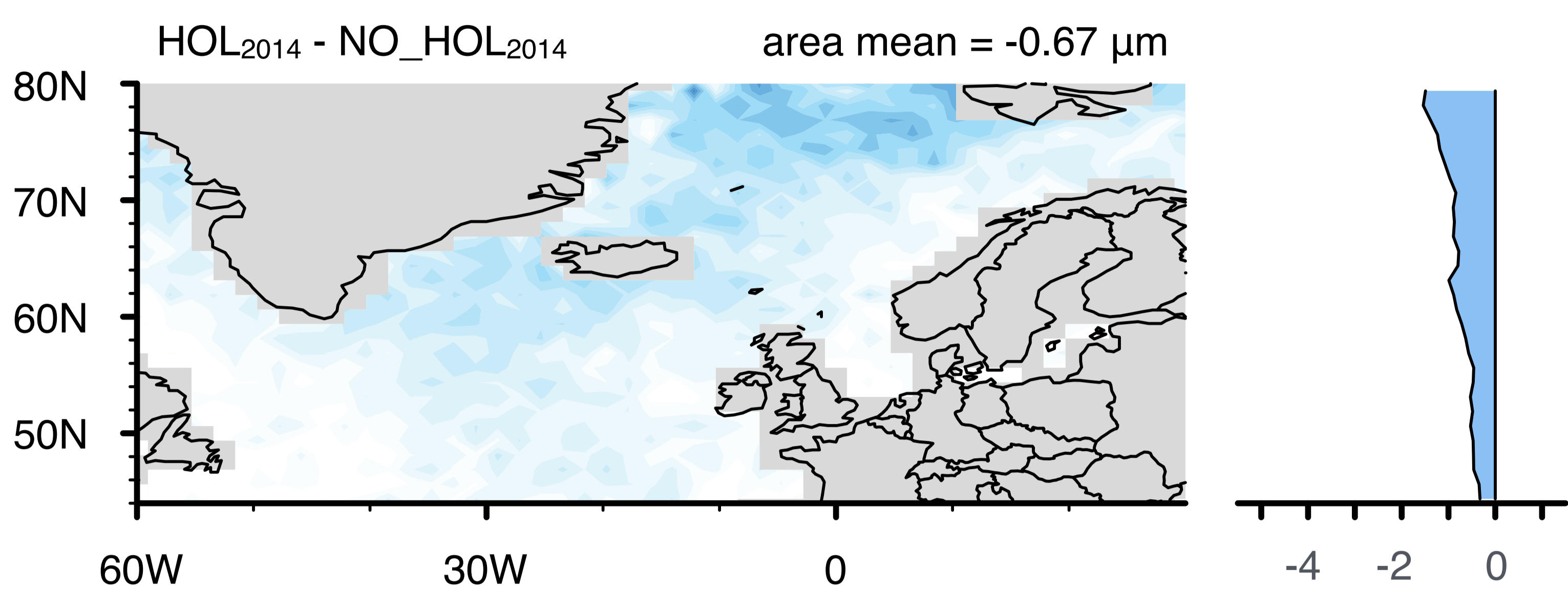
HadGEM3-CLASSIC
