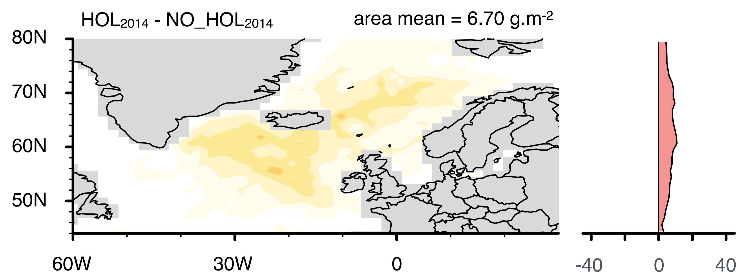
CAM5-NCAR
