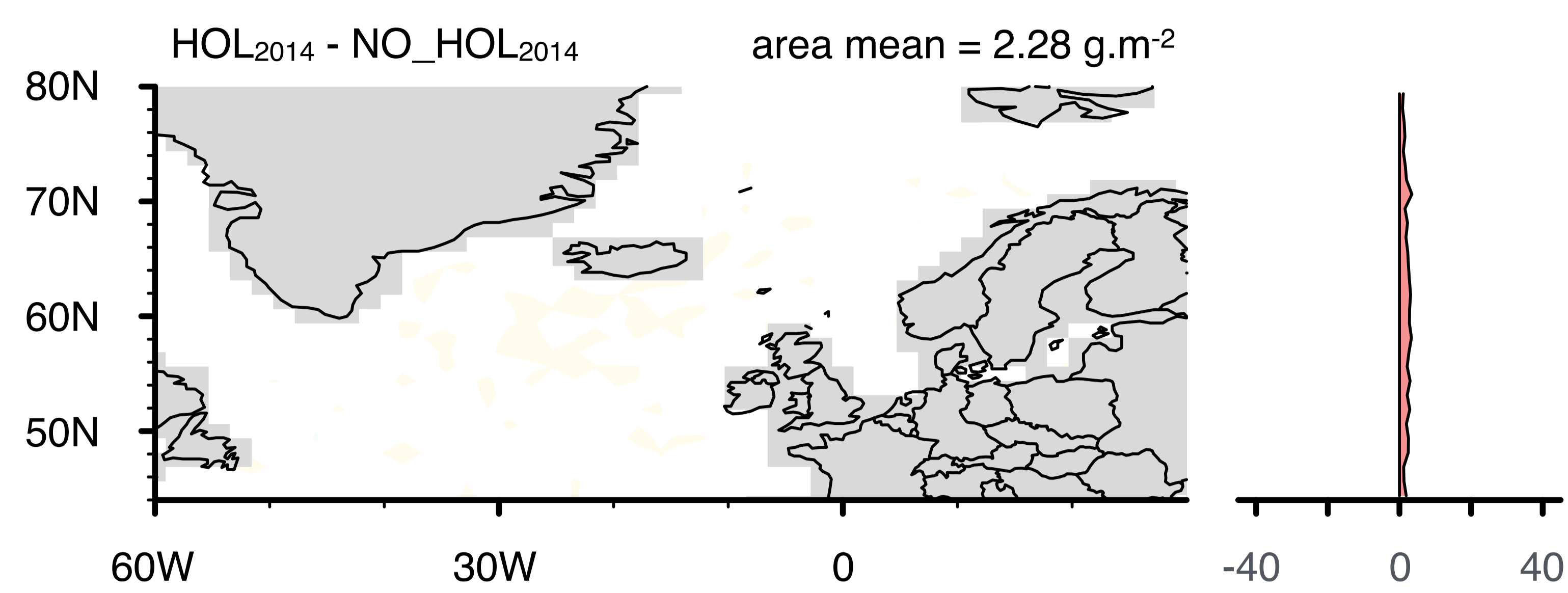
HadGEM3-CLASSIC
