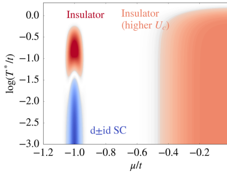
FIG. 1. Phase diagram of twisted bilayer graphene near the magic angle as a function of the temperature and chemical potential. Interactions U/t = 2 drive the system into various competing, strongly correlated phases: Near half filling of the lower band ( \mu \sim -t ), we observe a crossover between d + id superconductivity and AFM insulating behavior as T is increased. Near charge neutrality ( \mu = 0 ), the system is driven towards an AFM insulator, which, however, features a much higher critical interaction and becomes more pronounced only as U/t is increased (which can be achieved experimentally by tuning the twist angle).
