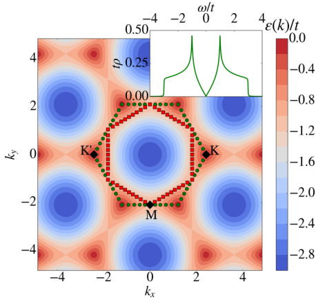
FIG. 2. Noninteracting dispersion relation of the lower band of twisted bilayer graphene as predicted by the Yuan-Fu model (1) [30]. The first Brillouin zone is marked by green dots. Near half filling of the lower band ( \mu \sim -t ), the Fermi surface (red squares) is both highly nested and contains a van Hove singularity in the density of states \rho (shown as the inset).
