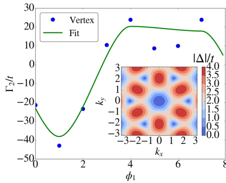
FIG. 4. Main panel: Fit of the effective coupling constant \Gamma_2 near \mu = -t along the dominant diagonal \vec{k}_1 + \vec{k}_2 = 0 to the form factors d_{x^2-y^2} and d_{xy} . Inset: Absolute value of the gap function (modulo an overall factor) for the mean-field solution that minimizes the minimal grand canonical potential. The gap is large at the van Hove points (which minimizes the grand free energy).
