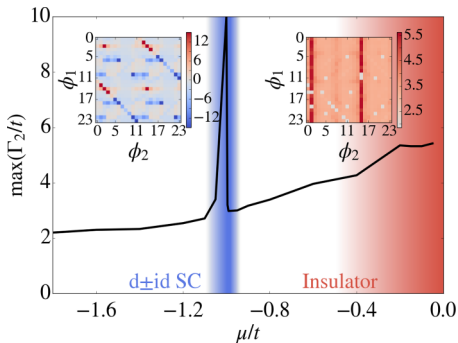
FIG. 3. Main panel: Maximum value of the effective coupling constant \Gamma_2^\Lambda at the end of the RG flow (fixed \Lambda_{\text{final}} = 10^{-4}t ) as a function of the chemical potential for a bare interaction U/t = 2 . We observe a strong enhancement around \mu \sim -t , and the corresponding momentum structure of \Gamma_2 along the Fermi surface (left inset) suggests d -wave SC in this region (see the main text for details). Near \mu = 0 , we find a momentum structure that indicates AFM insulating behavior (right inset). The enhancement of \Gamma_2 is much smaller than for the SC but becomes more pronounced when U/t is increased.
