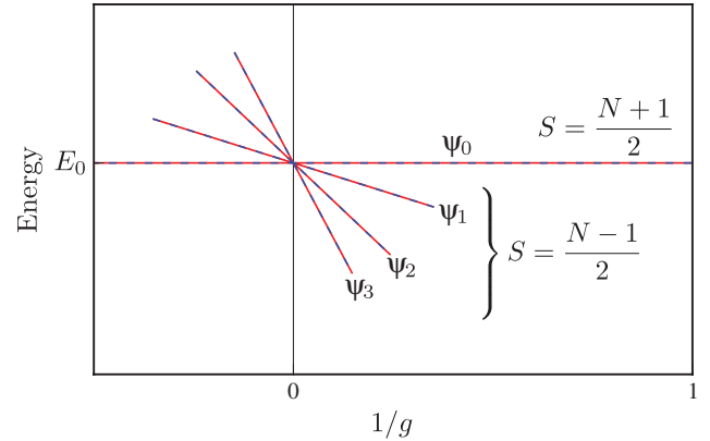
Fig. 1. Energy levels in the Tonks-Girardeau limit. We display the exact energies \langle \psi_l | \mathcal{H} | \psi_l \rangle (red) and the result of our ansatz \langle \tilde{\psi}_l | \mathcal{H} | \tilde{\psi}_l \rangle (blue dashed), given by E_0 - C_l/g in this limit, for the case of one \downarrow particle and N = 3 \uparrow particles. For g < 0 , there is also a two-body bound state at negative energies (not shown).
