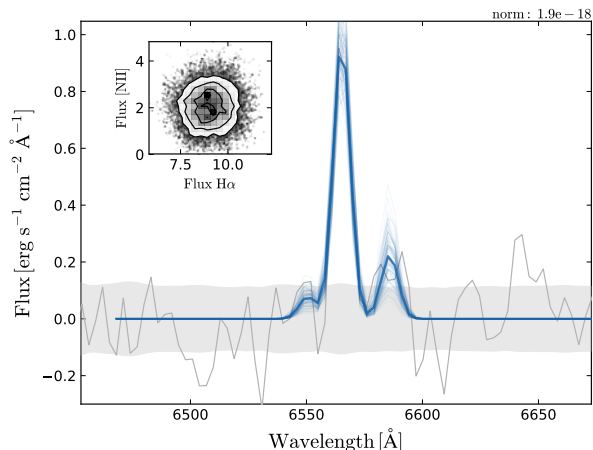
Fig. 1. Illustration of a fit to the H\alpha + [N II] \lambda\lambda 6548, 6584 emission line complex for the host of SNF20060912-004, a typical moderate signal-to-noise case. The gray line shows the emission line spectrum of the local host. The gray band represents its uncertainty, centered around zero. The thick blue line shows the best posterior estimation. The thin blue lines represent 100 realizations from the posterior distribution, illustrating the fit uncertainties. A posterior density sampling in the H\alpha versus [N II] flux plane is displayed as an inset.
