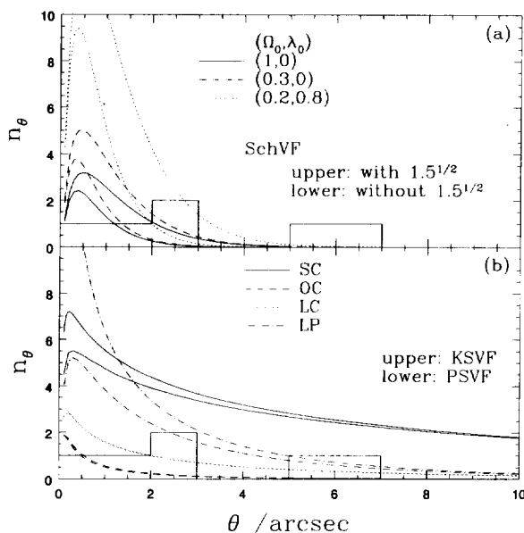
Fig. 3. Image separation distribution of the expected number of lensed QSO's in the HST survey. (a) Predictions from SchVF. (b) Predictions from PSVF and KSVF. Model parameters in (b) are listed in Table I. Histogram exhibits the observed distribution. SIS lens model ( \xi_c = 0 ) and the filled-beam distance ( \tilde{\alpha} = 1 ) are used.
