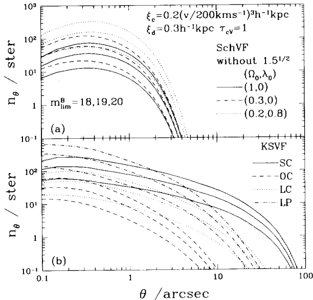
Fig. 8. Image separation \theta distribution of the expected number of all the lensed QSO's per unit steradian in the sky (Eq. (6.1)). (a) Predictions from SchVF. (b) Predictions from KSVF. From the lower to the upper of the three curves for each model, the limiting magnitude is m = 18, 19, 20 in B-band.
