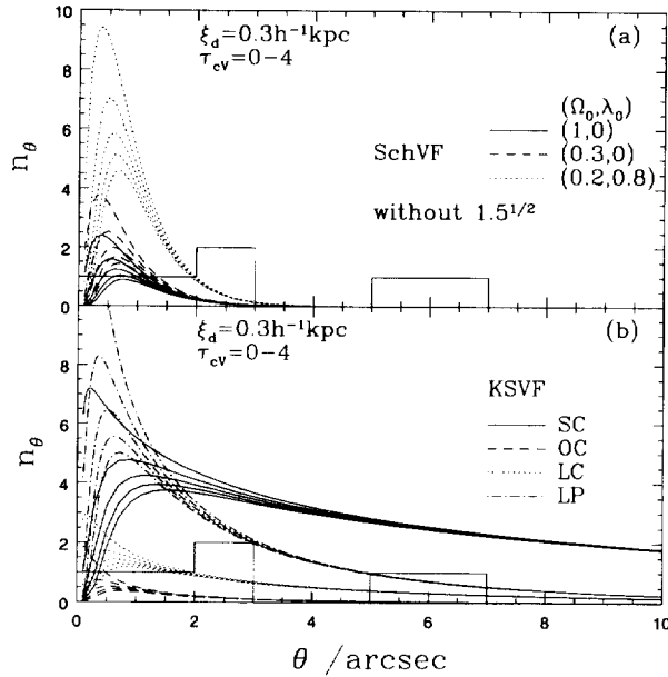
Fig. 7. Same as Fig. 3, except that the dust obscuration effect by lensing galaxies is included, and only KSVF predictions and SchVF predictions without the 1.5^{1/2} factor are shown. From the upper to the lower curves, the optical depth of the dust obscuration is \tau_{cv} = 0, 1, 2, 3, 4 (see Eq. (5-3)).
