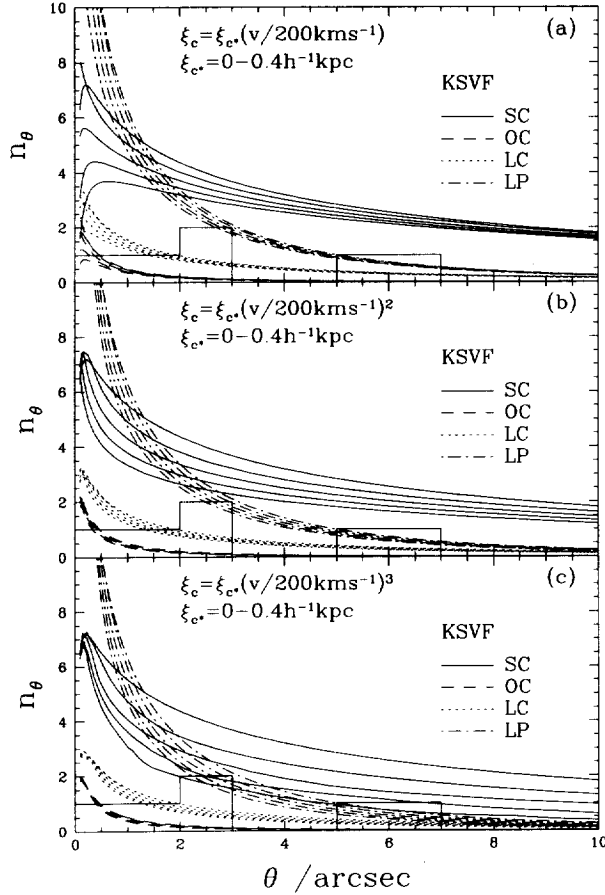
Fig. 5. Same as Fig. 3(b), except that the finite core radius \xi_c is included and only the KSVF predictions are shown. (a) \xi_c = \xi_{c*}(v/200 \text{ km s}^{-1}) ; (b) \xi_c = \xi_{c*}(v/200 \text{ km s}^{-1})^2 ; (c) \xi_c = \xi_{c*}(v/200 \text{ km s}^{-1})^3 ; with \xi_{c*} = 0, 0.1, 0.2, 0.3, 0.4 h^{-1} \text{ kpc} from the upper to the lower curves.
