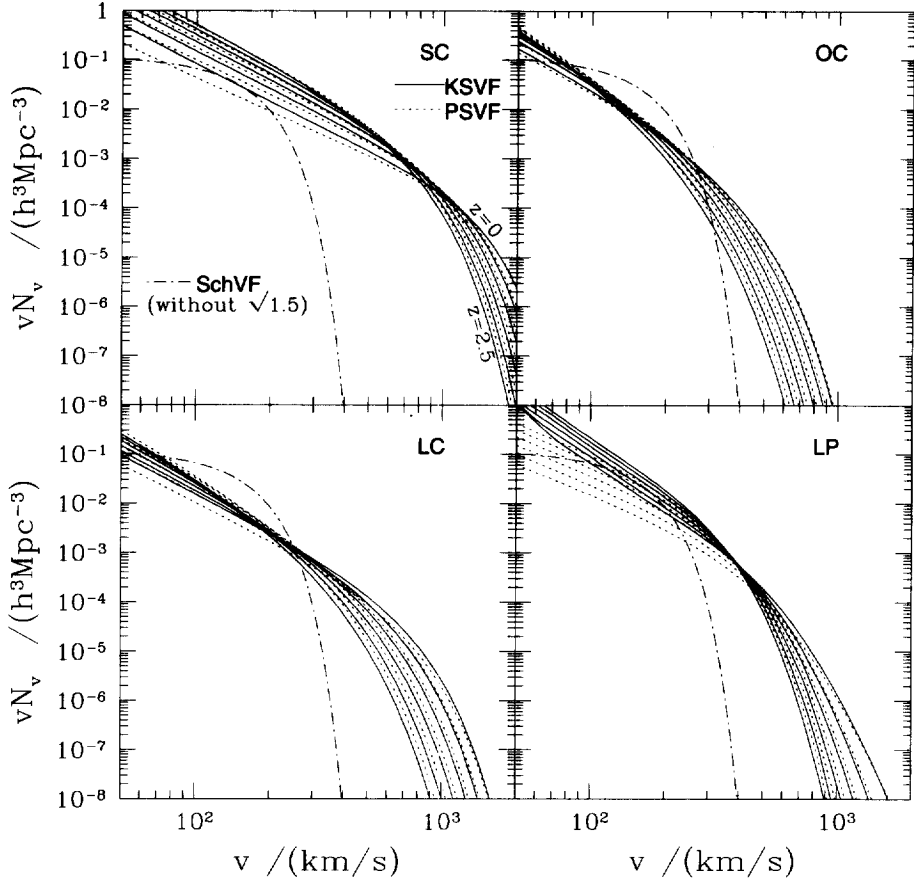
Fig. 2. Evolution of KSVF (solid) and PSVF (dotted) for the cosmological models listed in Table I. SchVF without 1.5^{1/2} is also shown in dot-dashed curve for reference. From the upper to the lower curves in high velocity end, z = 0, 0.5, 1, 1.5, 2, 2.5 .
