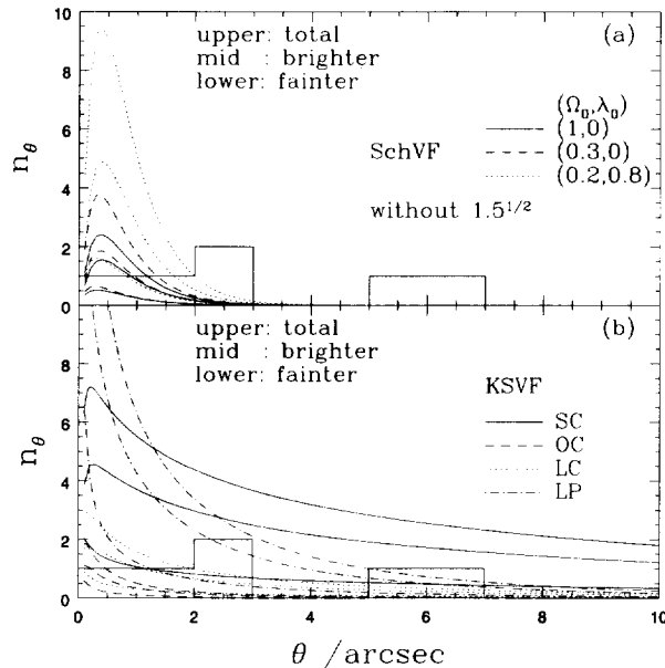
Fig. 6. Same as Fig. 3, except that \mu(y) in the magnification bias (2.21) is defined as the magnification of the brighter image (the middle curves) or the fainter image (the lower curves) of the outer two images. The upper curves use the total magnification of all the images for \mu(y) as in Fig. 3.
