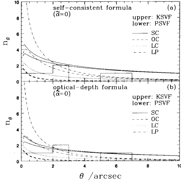
Fig. 4. Same as Fig. 3(b), except that the smoothness parameter (Eq. (2-10)) is \tilde{\alpha} = 0 . (a) Self-consistent formula (Eq. (2-15)) with the empty-beam distance ( \tilde{\alpha} = 0 ) is used; (b) optical-depth formula with the empty-beam distance ( \tilde{\alpha} = 0 ) is used instead of Eq. (2-15).
