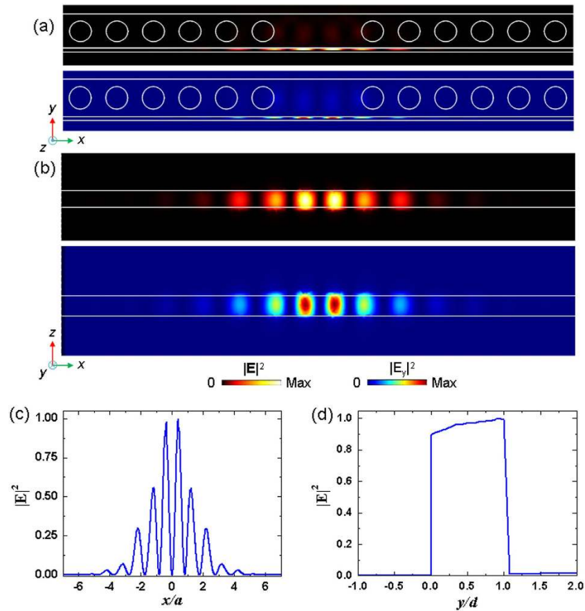
Figure 3. |E|^2 and |E_y|^2 field distributions of the SPP cavity mode on the (a) x-y and (b) x-z planes, respectively. The result is obtained using the supercell approach with seven lattice periods on each side of the cavity. The cavity mode is confined by the cavity and squeezed inside the air gap. Variations of the |E|^2 field for the cavity mode (c) at the center of the air gap along the x-direction and (d) close to the middle of the defect along the y-direction, respectively. In (c) x/a = 0 denotes the cavity center, and in (d) y/d = 0 denotes the silver substrate surface.
