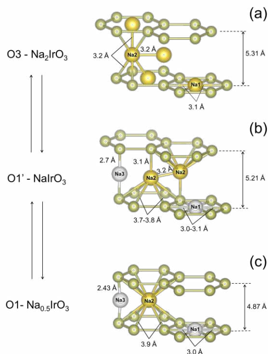
Figure 10. Possible Na positions for the pristine (a), O1' (b) and O1 (c) structures. Yellow atoms are the occupied positions and white balls represent sites left vacant with strong electrostatic repulsion from neighboring cations. Complete deintercalation of \text{Na}^+ in Na3 positions for the O1 structure cannot be achieved due to the very high stability of the site occupied by the last 0.5 Na.
