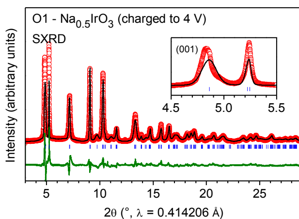
Figure 4. Rietveld refinement of synchrotron X-ray diffraction pattern for the fully charged \text{Na}_{0.5}\text{IrO}_3 (4V). The inset highlights the unusual shape of the first peak, which prevents a good refinement of the data.
