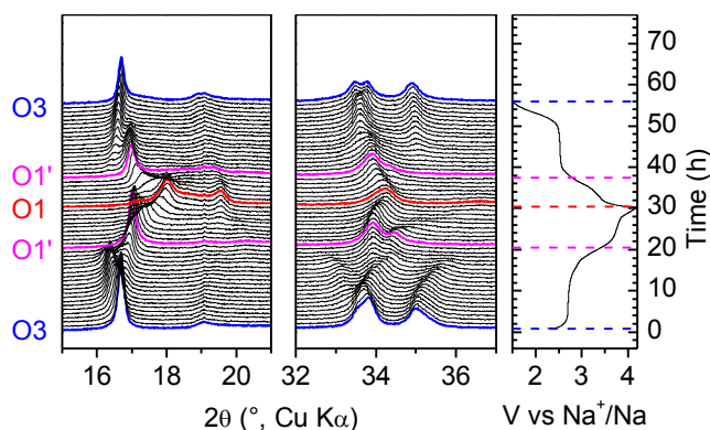
Figure 3. In situ XRD study of \text{Na}_2\text{IrO}_3 (cycled at C/40 between 1.5 V and 4 V). The pristine O3, O1' and O1 phases are highlighted in blue, pink and red, respectively.
