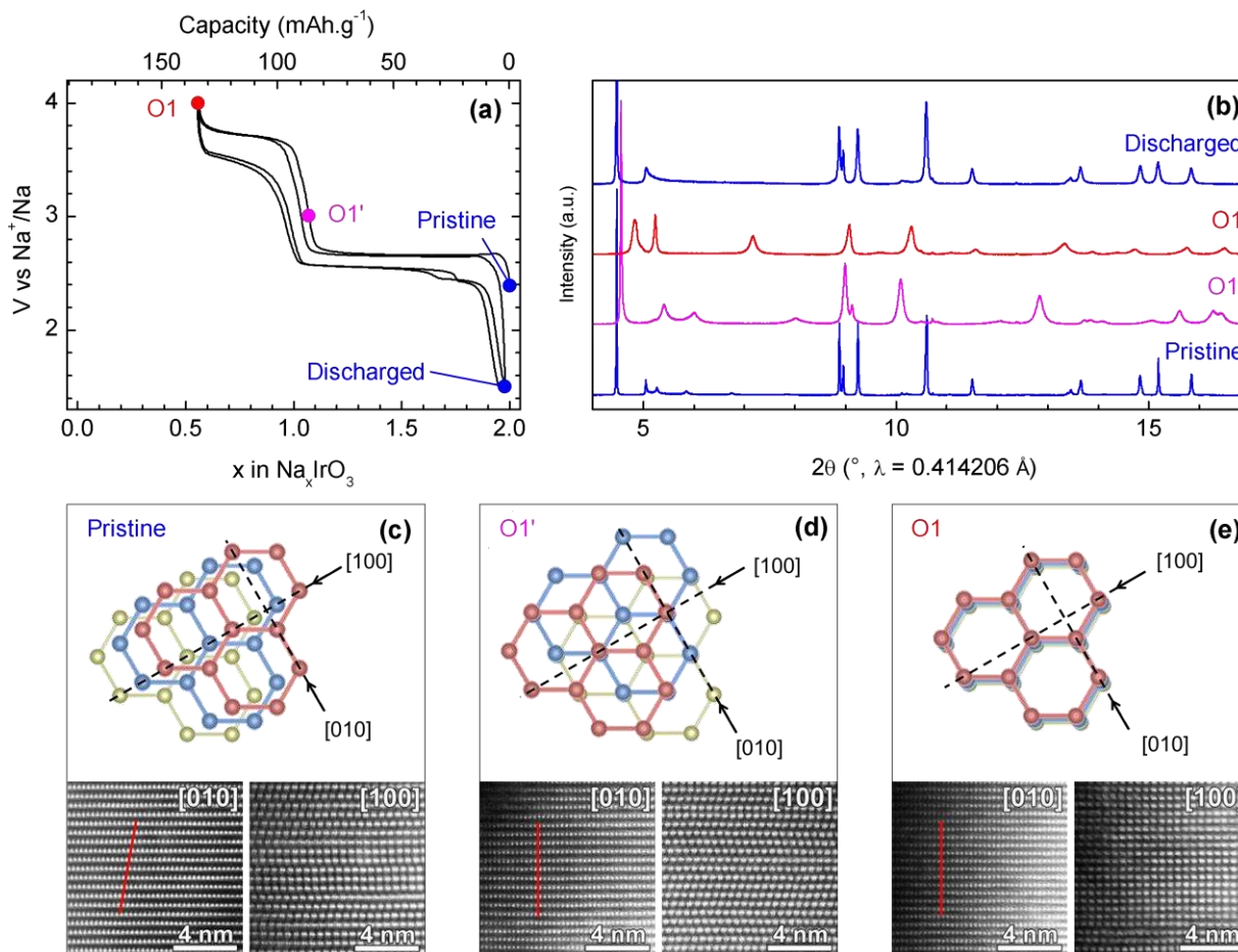
Figure 1. First and second galvanostatic cycles of Na 2 IrO 3 vs Na (a), SXR patterns (b) and high resolution HAADF-STEM images (c-e) of samples at different states of charge. Different stackings of the transition metal layers are found and represented here. For clarity, only the Ir honeycombs are represented in the sketch, and the crystallographic directions corresponding to the TEM observations are indicated. The red lines on the HAADF-STEM images highlight the perfect cubic close-packed ABCABC (c) and hexagonal close-packed ABAB (d, e) stacking of oxygen.
