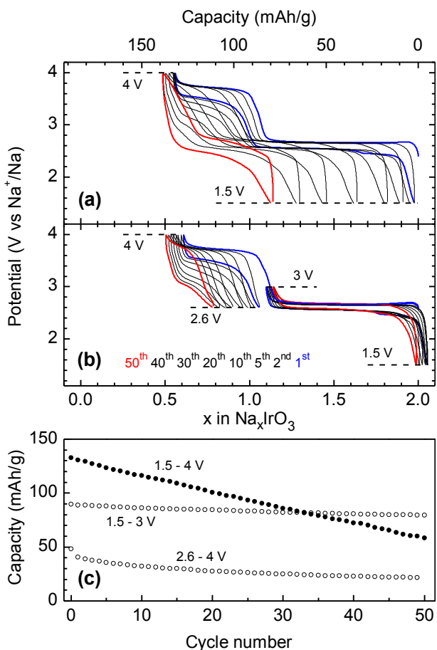
Figure 7. Galvanostatic cycling of Na 2 IrO 3 in Na half-cells (C/5 rate - 1 Na + in 5h) between 1.5 V and 4 V (a), on the lower or higher plateau (b) vs Na + /Na, using 1M NaClO 4 in EC:DMC with 1 % FEC as an electrolyte. First and 50 th cycles are highlighted in blue and red respectively. Capacity retention upon cycling for different cutoff voltages (c).
