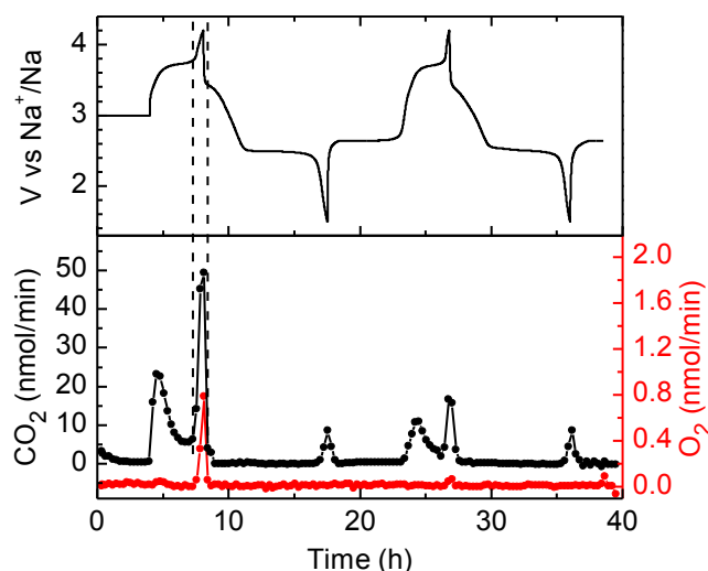
Figure 2. Online Electrochemical Mass Spectrometry data for the first and second cycles, with the voltage curve (a) and the evolution rate of CO 2 and O 2 indicated in black and red respectively (b). The cycling started from the material precharged at 3 V to limit degradation in air while preparing the electrode. A small amount of O 2 is detected at the very end of charge (between dashed lines).
