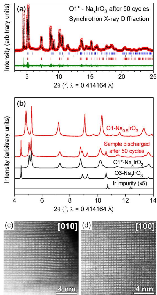
Figure 8. Synchrotron X-ray diffraction patterns for Na 2 IrO 3 discharged after 50 cycles (a). This fit was obtained with a 3 phases model where phase 1 (O3-Na 2 IrO 3 , blue ticks) and phase 2 (Ir impurity, black ticks) were refined using the Rietveld method, and phase 3 (O1*-Na x IrO 3 , red ticks) was fitted using pattern-matching. Comparison of the experimental pattern to the three isolated components and to the experimental pattern of O1-Na 0.5 IrO 3 (b). TEM data for the discharged sample after 50 cycles demonstrating stabilization of the O1 structure even in the discharged state (c-d).
