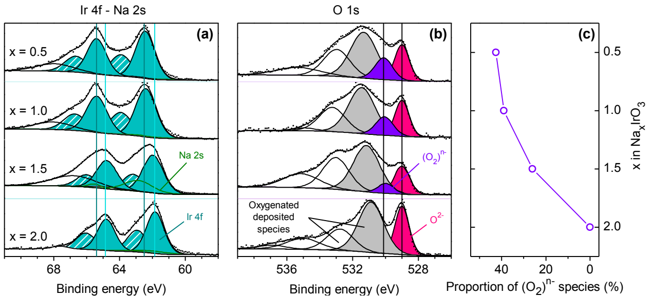
Figure 5. Modification of the oxidation states of Ir and O during the first charge. XPS analysis of Ir 4f (a) and O 1s (b) peaks show that both Ir and oxygen are oxidized on the first plateau, and oxygen only on the second plateau. The proportion of (O 2 ) n- species depending on state of charge is shown in (c).
