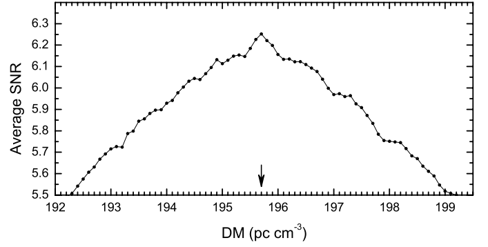
Fig. 3. Variation of average SNR with DM . The average SNR that has a peak value at DM = 195.7 pc cm ^{-3} as indicated by the arrow, is calculated from all 423 detected bursts from RRAT J1819–1458 with DM increasing from 192 to 199.5 pc cm ^{-3} in steps of 0.1 pc cm ^{-3} .
