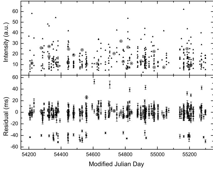
Fig. 4. Variation in flux intensity with date ( top ) and timing residuals ( bottom ) for RRAT J1819–1458. The flux intensity is measured in an arbitrary unit and no remarkable deviation of flux density is shown in the variation plot. The timing residuals that show a distribution of three bands with \sim 40 ms intervals are calculated with the fitted parameters listed in Table 1. The rms of residuals is 17 ms and the error bars are 10\sigma . Dots with circles in the graphs are the counterparts of bimodal bursts and the gaps in date are due to observation scheduling.
