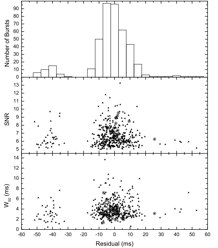
Fig. 5. Distribution of timing residuals of 423 detected bursts from RRAT J1819–1458 ( top ), and, plots of SNR ( middle ) and W_{50} ( bottom ) versus timing residual. Circles in the two plots are the counterparts of bimodal bursts.
