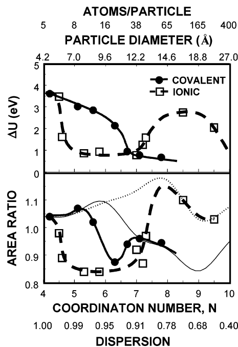
Figure 7. Comparison of the experimental \Delta U and the area ratio R = A(\Delta VB_c)/A(\Delta VB_b) as a function of the Pt–Pt coordination number N for covalent or acidic (solid lines) and ionic or basic (dashed lines) supports. The N values were obtained from EXAFS analyses summarized elsewhere. 10,11,17,18 Also plotted are the optimum R_{\text{noICT}}(N) (light dashed line) results obtained from eq 4. The horizontal axis shows the estimated dispersion, cluster diameter, and number of atoms/particle as estimated assuming spherical clusters and fcc packing (see the text). Data shown include those for covalent (acidic) supports (i.e., for LTL[K/Al]=0.63] zeolite and \text{Cl-Al}_2\text{O}_3 , \text{SiO}_2 ) and for ionic (basic) supports (LTL[K/Al]=1.25] zeolite and \text{K-Al}_2\text{O}_3 , \text{K-SiO}_2 ). The uncertainty in N , U , and R is estimated as follows: \delta N = \pm 0.2 , \delta U = \pm 0.3 , and \delta R = \pm 0.1 .
