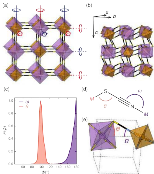
Fig. 2 (a) Illustration of the tilt system of \text{Fe}[\text{Bi}(\text{SCN})_6] shown on the hypothetical Fm\bar{3}m aristotype: red indicates clockwise and blue indicates anticlockwise. In-phase ( k=0 ) tilts are indicated by solid lines, anti-phase tilts ( i.e. k = \frac{1}{2} ) are indicated by dashed lines. (b) The actual crystal structure of \text{Fe}[\text{Bi}(\text{SCN})_6] shown at the same scale. Its unit cell is shown by black, dashed lines. (c) Distribution of the M-X-C angle for N- and S-bound thiocyanate, determined via database search in the CSD. There is a clear preference for linear M-NCS and bent M-SCN bonds. (d) Definition of relevant bond and tilt angles. Pseudo-cubic unit cell shown in dashed lines.
