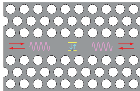
FIG. 1 (color). Schematics of the system. A two-level system is coupled to a one-dimensional continuum in which the photons, shown as wiggly waves, propagate in each direction.
