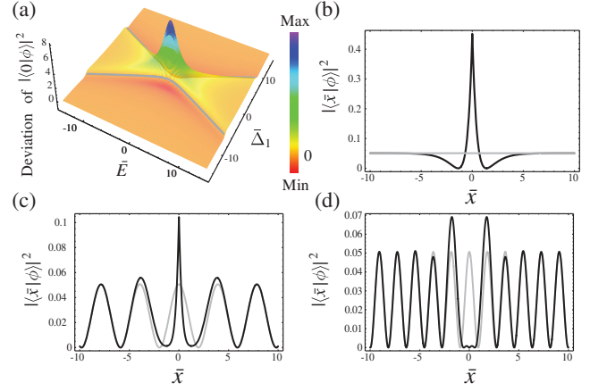
FIG. 3 (color). (a) Plot of the normalized deviation of the relative wave function: |\langle \bar{x}=0 | \phi \rangle|^2 / (\sqrt{2}/2\pi)^2 - 1 . \bar{x} \equiv (\Gamma/2)x . The two gray lines indicate the zero value. (b)–(d) Plots of |\langle \bar{x} | \phi \rangle|^2 for \bar{E}_1 = 0 . (b) \bar{\Delta}_1 = 0 , (c) \bar{\Delta}_1 = -0.8 , (d) \bar{\Delta}_1 = -\sqrt{3} . Gray lines indicate the interaction-free case.
