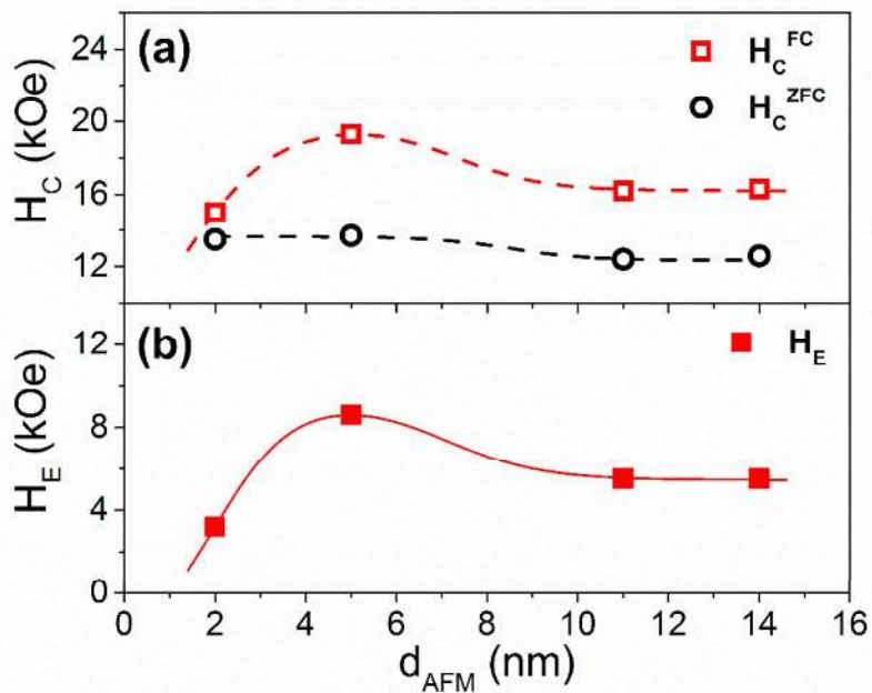
Figure 5. (a) H_C at 10 K as a function of d_{AFM} ; H_C values were obtained after FC at 120 kOe (red) or ZFC (black) processes from RT. (b) H_E at 10 K as a function of d_{AFM} after FC at 120 kOe process from RT. (The lines are guides to the eyes).
