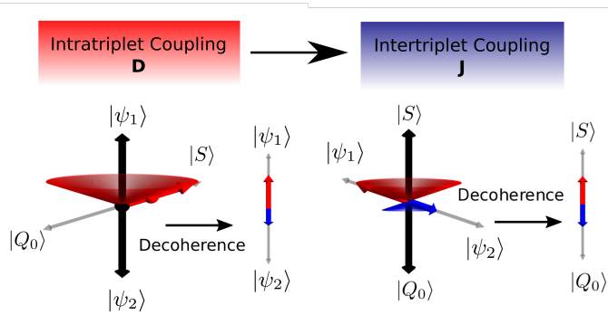
Figure 5: Quintet formation through time-dependent exchange interaction. A time-dependent exchange coupling enables decoherence from the weak-exchange singlet/quintet pair eigenstates |\psi_1\rangle and |\psi_2\rangle into the strong-exchange-coupled quintet |Q_0\rangle eigenstate. The transition from a weak to a strong exchange interaction drives the formation of the pure quintet pair state |Q_0\rangle .
