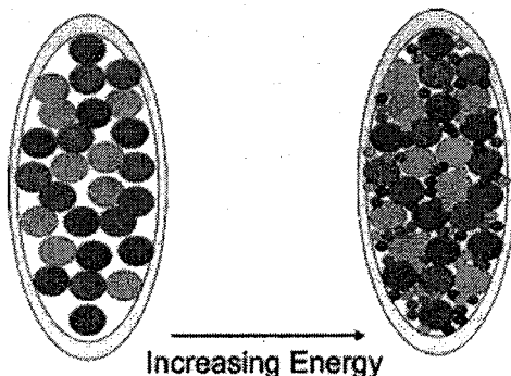
Figure 11: More gluons added to a hadron as the hadron energy increases..
