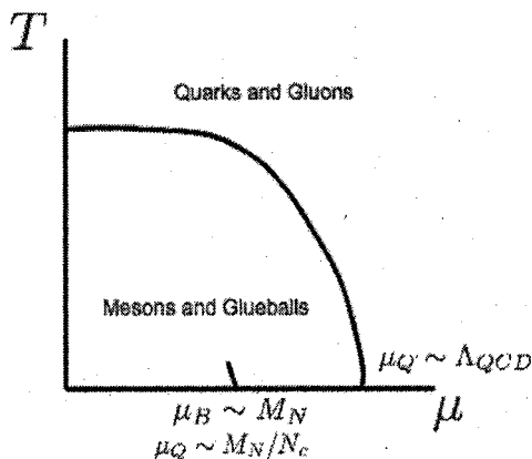
Figure 8: The popular folklore for the phase diagram of QCD.
