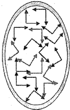
Figure 12: The color electric and color magnetic fields in the Color Glass Condensate.
