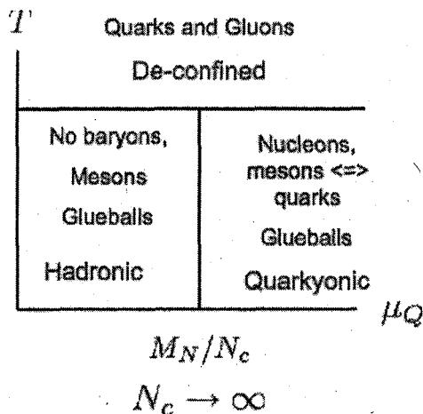
Figure 9: The phase diagram of QCD at large N_c .
