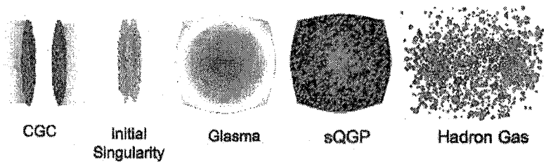
Figure 1: A schematic picture of the evolution of matter produced in the heavy ion collisions.
