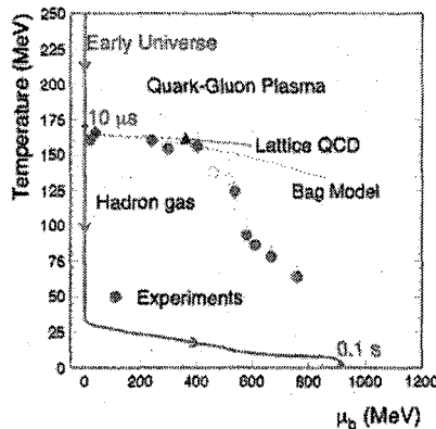
Figure 10: Freeze out temperature and baryon chemical potential determined by heavy ion collisions.
