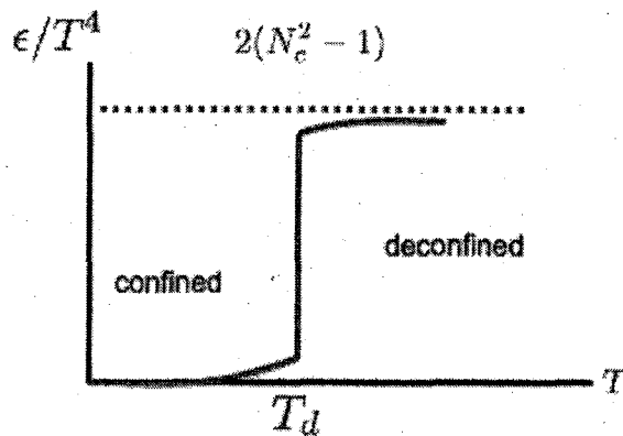
Figure 3: The energy density scaled by T^4 for QCD in the absence of dynamical quarks.
