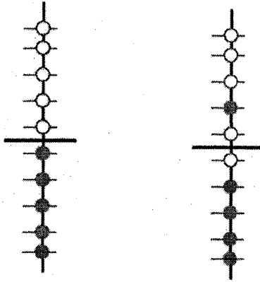
Figure 7: The energy levels of the Dirac equation. Unfilled states are open circles and filled states are solid circles. For the free Dirac equation, negative energy states are filled and positive energy states are unoccupied, as shown on the left hand side. A mesonic excitation corresponding to a particle hole pair is shown on the right hand side.
