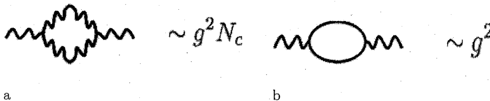
Figure 5: a: The gluon loop contribution to the heavy quark potential. b: The quark loop contribution to the potential
