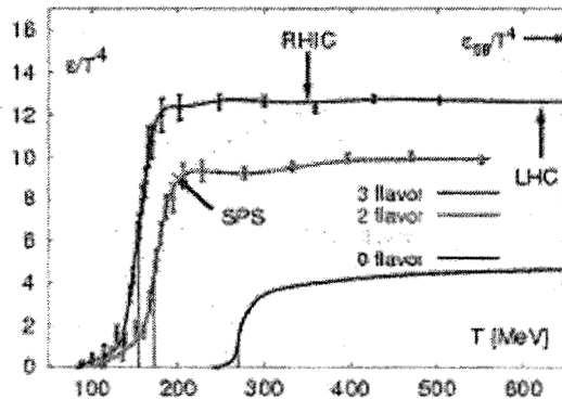
Figure 4: The energy density scaled by T^4 measured in QCD from lattice Monte Carlo simulation. Here there are quarks with realistic masses.
