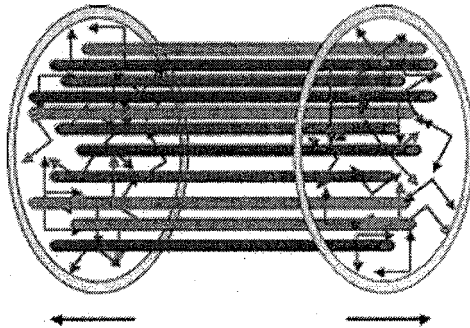
Figure 13: The color electric and color magnetic fields of the Glasma immediately after the collision of two hadrons.
