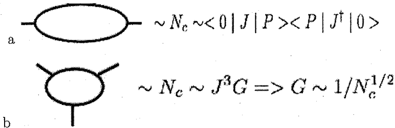
Figure 6: a: The quark loop corresponding to a current-current interaction. b: A quark loop corresponding to a three current interaction.
