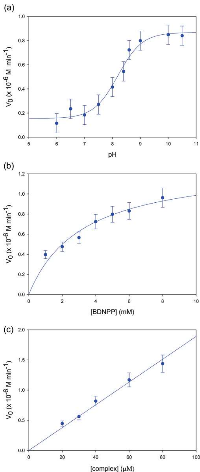
Figure 2. Catalytic properties of [\text{Mn(II)Mn(III)(L1)(OAc)}_2]\text{ClO}_4 \cdot \text{H}_2\text{O} . (a) pH dependence (5 mM substrate); (b) substrate dependence at pH 10; (c) complex dependence at pH 10.
