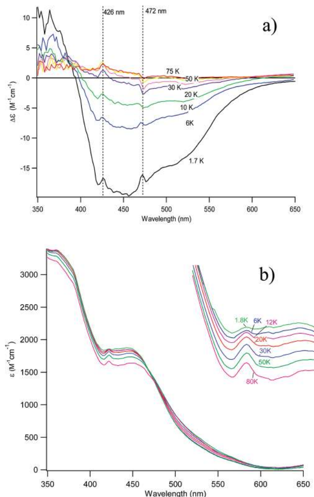
Figure 5. (a) Variable temperature MCD spectra of [Mn(II)-Mn(III)(L1)(OAc) 2 ](ClO 4 ) measured at 5 T in a methanol/ethanol glass. (b) Variable temperature absorption spectra of [Mn(II)Mn(III)-(L1)(OAc) 2 ](ClO 4 ) in a methanol/ethanol glass. Inset shows the 400–450 nm region, with the temperatures as shown.
