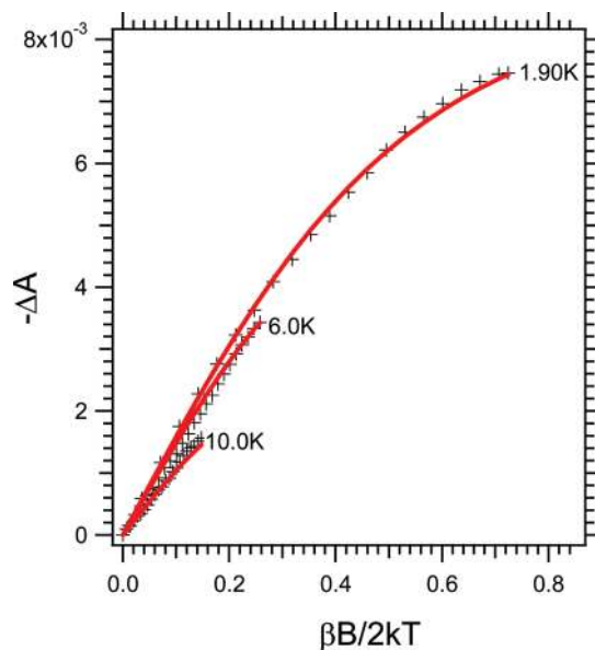
Figure 6. VTVH MCD data of [Mn(II)Mn(III)(L1)(OAc) 2 ](ClO 4 ) in a methanol/ethanol glass. Solid lines indicate the fit to the data using J = -4.7 \text{ cm}^{-1}, D(\text{Mn(III)}) = 4.3 \text{ cm}^{-1} .
