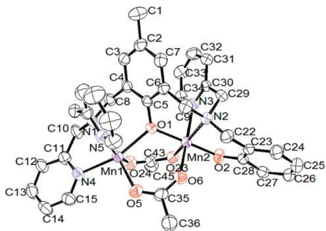
Figure 1. ORTEP plot of [\text{Mn(II)Mn(III)(L1)(OAc)}_2]^+ cation. Thermal ellipsoids are shown at 30% probability, hydrogen atoms are excluded for clarity. The bond lengths are Mn1–O5 = 2.070(4) Å, Mn1–O24 = 2.144(4) Å, Mn1–O1 = 2.192(3) Å, Mn1–N4 = 2.252(5) Å, Mn1–N5 = 2.288(5) Å, Mn1–N1 = 2.297(4) Å and Mn2–O2 = 1.839(3) Å, Mn2–O1 = 1.925(3) Å, Mn2–O23 = 1.985(4) Å, Mn2–N2 = 2.120(4) Å, Mn2–O6 = 2.145(4) Å, Mn2–N3 = 2.271(4) Å where Mn1 and Mn2 denote the Mn(II) and Mn(III) centers, respectively.
