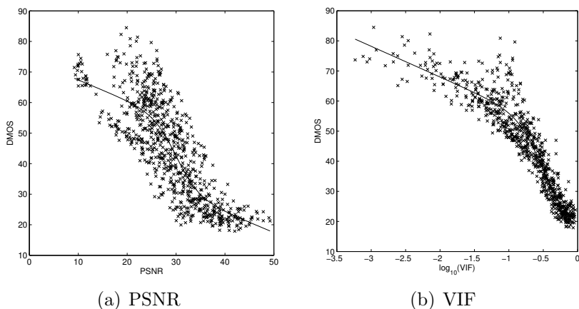
Figure 9: VIF: Plot of DMOS vs. model prediction and the best fitting logistic function to the subjective and objective scores [Reproduced from [12]]
