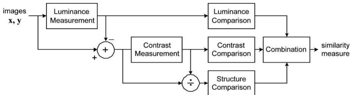
Figure 4: Block Diagram of the SSIM Quality Assessment System [Reproduced from [10]]
