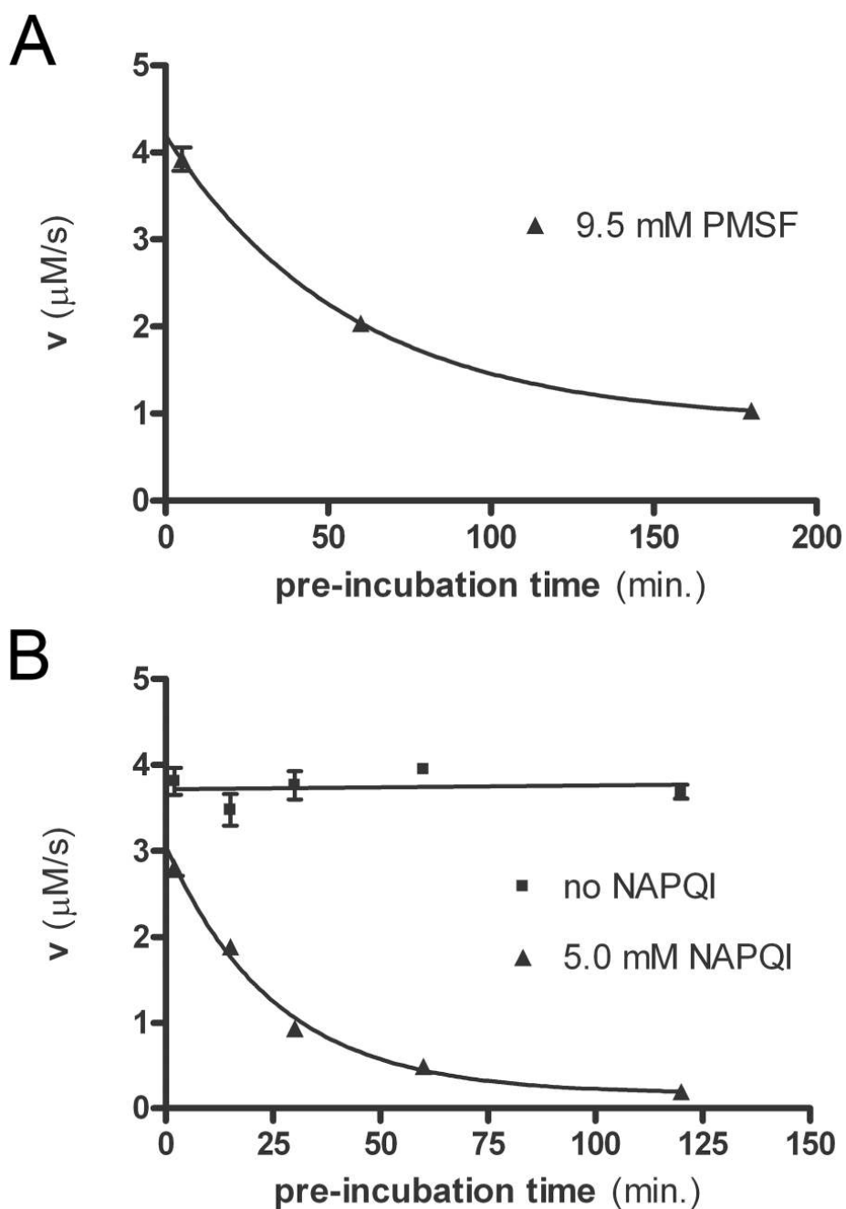
Figure 1. Kinetic Analysis Reveals Time-Dependent Inhibition of MIF by both PMSF and NAPQI. HPP tautomerase activity of MIF was measured after various times of incubation with (A) PMSF or (B) NAPQI. Inhibitor concentrations shown are those during the incubations, and were in 48-fold molar excess of MIF. After incubation with inhibitor, the MIF solution was diluted to 0.2 \mu\text{M} MIF in tautomerase assay buffer and activity was measured. Data shown are from triplicate experiments. Mean \pm SEM are plotted for all data. For many points, the error bars are too small to be seen beyond the data point symbol.
