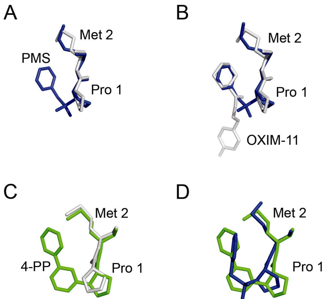
Figure 5. Flexibility of PMS allows binding to MIF with only minimal protein conformational change. A, B. Overlays of the PMS-MIF structure onto ( A ) unliganded MIF and ( B ) MIF bound to OXIM-11 (PDB entry 2OOH) (3). In both panels, the PMS-MIF structure is in blue. C, D. Overlay of ( C ) unliganded MIF (white) and ( D ) PMS-MIF (blue) onto MIF bound by the less flexible covalently bound ligand 4-PP (PDB entry 3B9S, green) (40).
