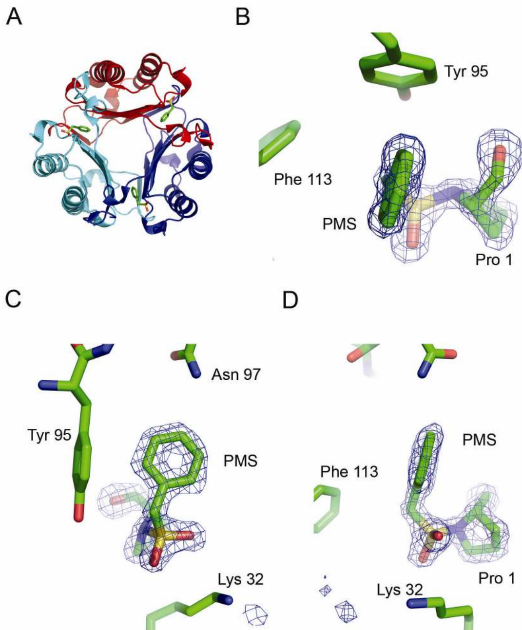
Figure 4. Crystallographic Structure of PMS-MIF Complex at 1.55\text{\AA} . A . Global structure of the PMS-MIF complex. B , C , D . Active site with 4.5\sigma F_o-F_c electron density calculated omitting Pro 1 and the PMS moiety. The fit to the electron density is displayed in active site A and is similar in the other two active sites. B . View showing the tetrahedral character of the Pro 1 nitrogen. C . View showing phenyl ring of PMS in active site. D . Same as (C), but rotated 90^\circ , showing the covalent bond between Pro 1 and the PMS moiety.
