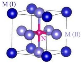
FIG. 1. Structure of M_4N compound with M = \text{Fe, Co, Ni, Mn} . The two inequivalent metal sites M(\text{I}) and M(\text{II}) adopt an antiperovskite structure as M(\text{I})M(\text{II})_3N .
