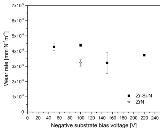
Fig. 11 The specific wear rate of Zr-Si-N coatings as a function of negative substrate bias voltage
