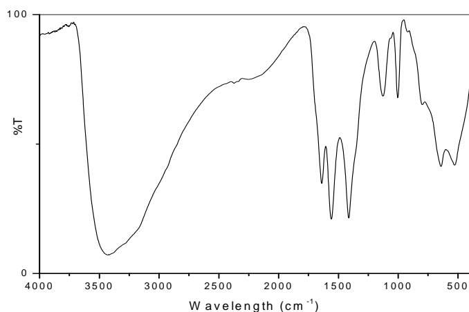
Fig. 3 FTIR spectrum of ZnS nanoparticles
