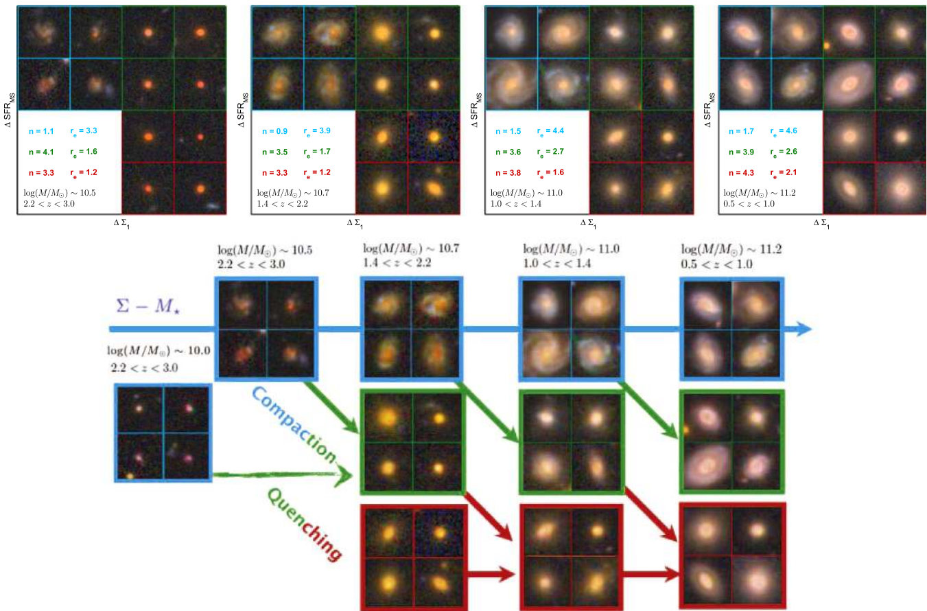
Figure 9. Top: snapshots of galaxies in the different phases of the evolutionary sequence in \Delta\SFR - \Delta\Sigma_1^Q (see Figure 6): extended SFGs (blue), compact SFGs (green) and quiescent galaxies (red). Each panel shows galaxies with increasing stellar masses as a function of time (left to right) following the mass growth track from z = 3 to z = 0.5 in Behroozi et al. (2013). The numbers in the bottom-left inset indicate the median n and r_e of the galaxies in each group. Bottom: examples of possible evolutionary pathways following the mass growth track with redshift. For the same mass growth, some SFGs may remain in the SFR–MS, since from z = 3 to z = 0.5 , they are growing in size and central density, and acquiring progressively more settled disk-like appearances (blue), while others would experience a faster core growth, relative to the latter, resulting in a strong increase in \Sigma_1 and \Sigma_e (green). The compaction and quenching processes are likely entwined, and once both are started, the complete shutdown of star formation takes place after galaxies have reached a maximum central density, showing only minor changes in their structural and visual appearances relative to their compact SFG progenitors (red).
