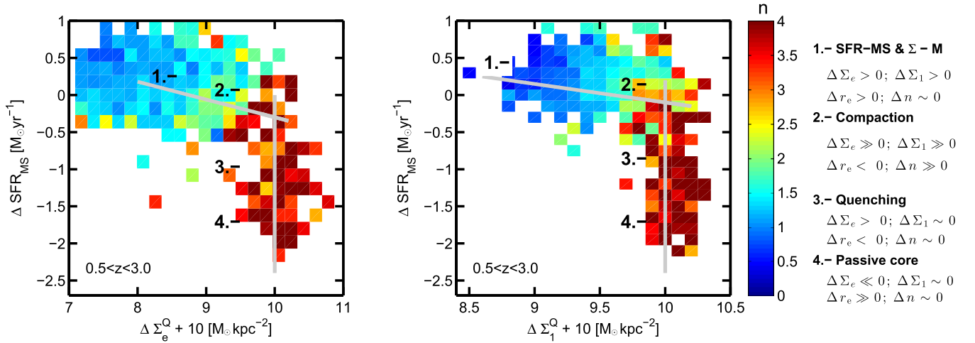
Figure 7. Stacked \Delta \text{SFR}_{\text{MS}} vs. \Delta \Sigma_e^Q (left) and \Delta \Sigma_1^Q (right) for all massive galaxies at 0.5 < z < 3 , color-coded by the Sérsic index. The distribution shows all galaxies in Figure 6 after correcting for the zero-point evolution of the structural relations and normalized at \log A = \log B = 10 M_{\odot} \text{ kpc}^{-2} . The gray lines show the best-fit linear relations for SFGs and quiescent galaxies. The numbers and the legend on the right side of the panel summarize the approximate evolutionary phases along the L-shape sequence: (1) the inside-out growth of a SFG in the SFR–MS, which increases both its effective radius and central mass at a relatively constant Sérsic index (i.e., disk growth); (2) a phase of enhanced core growth, relative to the previous phase, which increases the Sérsic index; the slight tilt of the steps 1–2 suggests that the onset of quenching goes hand in hand with the compaction process; (3) a complete shutdown of star formation at maximum \Sigma_e and \Sigma_1 in compact SFGs; and (4) a passive phase in which \Sigma_1 remains relatively constant while \Sigma_e decreases quickly due to size growth and the quenching of new (larger) galaxies.
