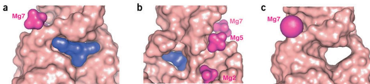
Figure 4 Surface representation of the catalytic pocket. (a,b) Front (a) and back (b) views of the catalytic pocket of the ribozyme–product complex. (c) Front view of the free ribozyme. Mg^{2+} ions are shown as hydrated cations in a and b for the 3.0-Å structure, and as balls in c for the 3.5-Å structure.
