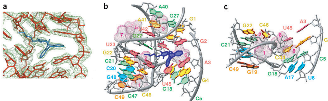
Figure 2 Details of the structure of the Diels-Alder ribozyme-product complex. (a) Final 2F_o - F_c electron density map (green), contoured at 1 \sigma , for the cycloaddition product and surrounding RNA. The product (blue) and RNA (red), superimposed with the density, are from the refined model. (b) RNA tertiary structure surrounding the ribozyme catalytic pocket containing bound product. The product is blue, adjacent A3-U45 and U23•A43 base pairs and U42•(G2-C25) base triple are light red, G24 is green, with additional layers moving farther out from the pocket in gold (A41•(C26-G2), G22-C46 and C44-G4), light green (A40•G27, C21-G47 and G18-C5), cyan (C20-G48) and orange (G19-C49). The hydrated Mg^{2+} cations are in magenta-colored mesh. (c) Tertiary structure in the region of stems I and II. The RNA is slightly tilted compared with b to highlight the relative alignment of the stems. Individual base pairs and hydrated Mg^{2+} cations are shown as in b .
