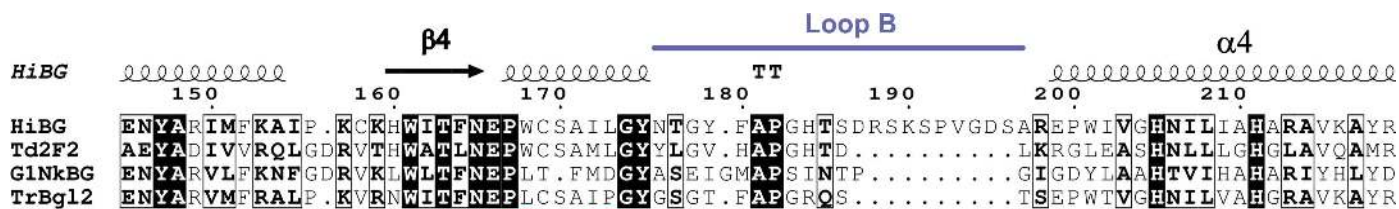
Figure 6 Sequence alignment of GH1 \beta -glucosidases with different levels of glucose tolerance. HiBG, H. insolens \beta -glucosidase (BG); Td2F2, BG from a compost metagenomic library (GenBank accession No. HV538882); G1NkBG, N. koshunensis BG1 (GenBank accession No. AB073638); TrBgl2, T. reesei BG2 (NCBI accession No. AB003110). Red spots indicate amino-acid positions that seem to play a role in glucose tolerance. Trp168 and Leu173 of HiBG are conserved in Td2F2; both are glucose-tolerant enzymes ( \geq 450 \text{ mM} ). When mutated at these positions (Leu167Trp and Pro172Leu), TrBgl2 (glucose K_i = 48.5 \text{ mM} ) showed increased glucose tolerance (3.0-fold and 1.6-fold, respectively; Lee et al. , 2012).
