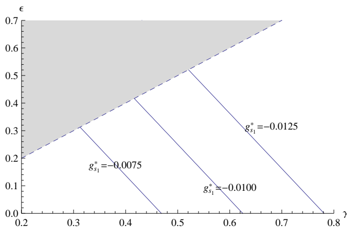
Figure 6: \gamma and \epsilon combinations perfectly matching the structural change
