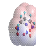
1 RDX
