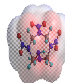
HMX-Hydroxylamine
