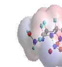
3 HydroxAmRDX
