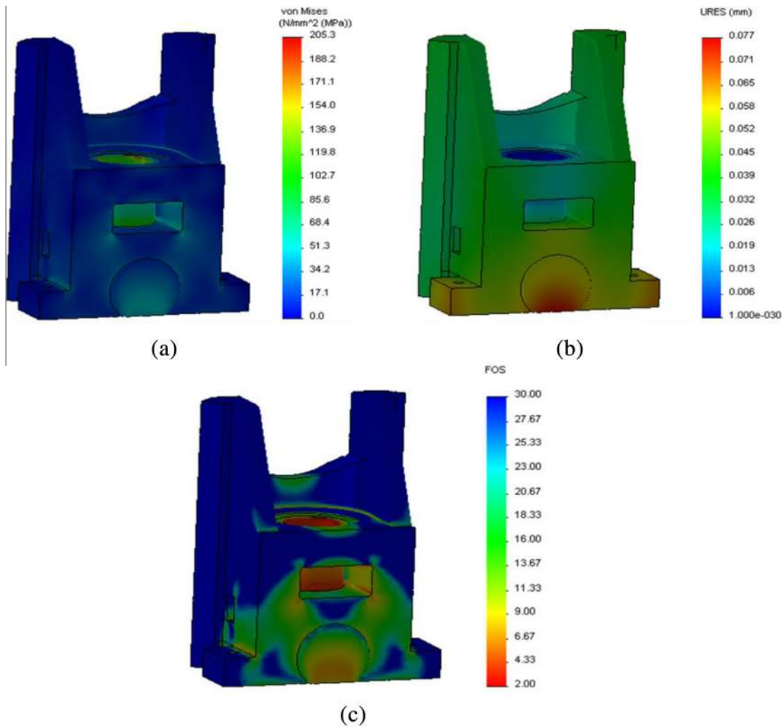
Fig. 10. Structural analysis results of the ram assembly: (a) von-Mises stress, (b) Deformation, (c) Factor of safety.
