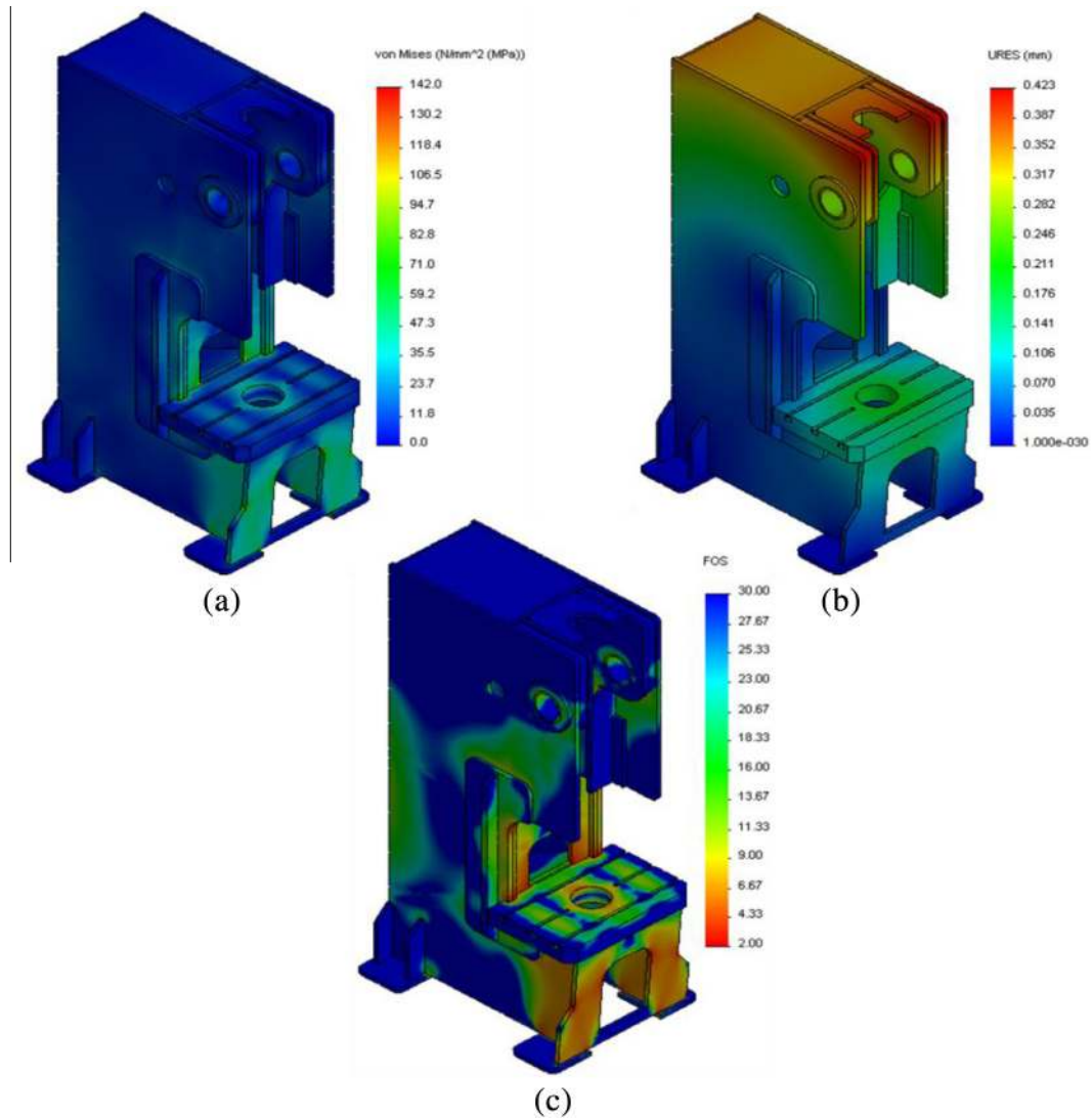
Fig. 12. Structural analysis results of the main body assembly: (a) von-Mises stress, (b) Deformation, (c) Factor of safety.
